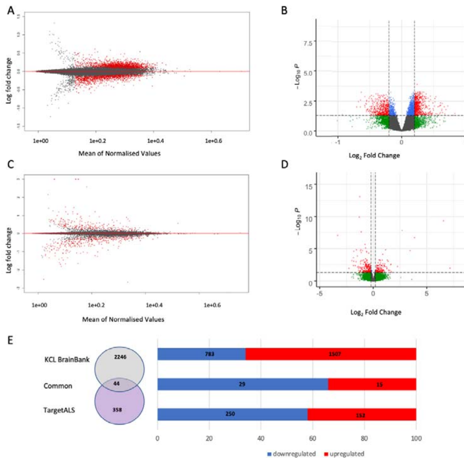
Figure 1. A) KCL BrainBank and C) TargetALS MA plots representing the distribution of \log_2 fold change ( \log_2FC ) across all expression levels; B) KCL BrainBank and D) TargetALS Volcano plots. Plot D has been cropped to exclude one point with extremely high \log_2 fold change. Genes coloured red pass both the p -value and \log_2FC thresholds. Grey genes are not significant, green genes only pass the \log_2FC threshold, and blue genes only pass the \log_2FC threshold. E) Numbers of differentially expressed genes in the two datasets.
