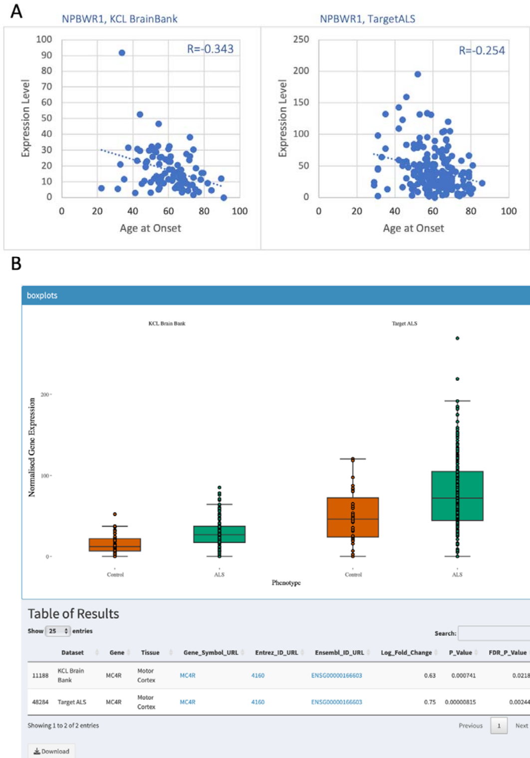
Figure 4: A) Correlation analysis between NPBWR1 gene expression and age of onset in KCL BrainBank and TargetALS. B) Screenshot from ALS Gene Expression Explorer showing expression of MC4R , which was significantly upregulated in both datasets.
