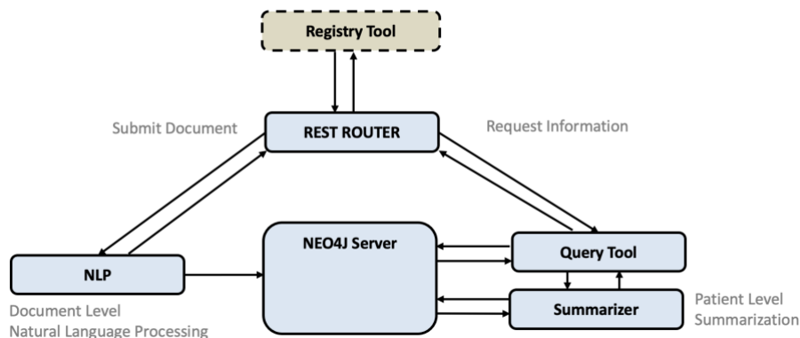
Figure 1: The DeepPhe-CR architecture
