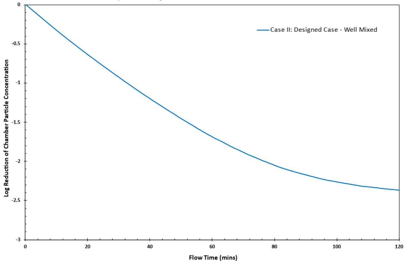
Figure 11. Total reduction of particles inside the designed ventilation system test chamber with one inlet pipe and one outlet pipe unit inside the room. The airflow inside the room was designed to operate at 2000 CFM.
