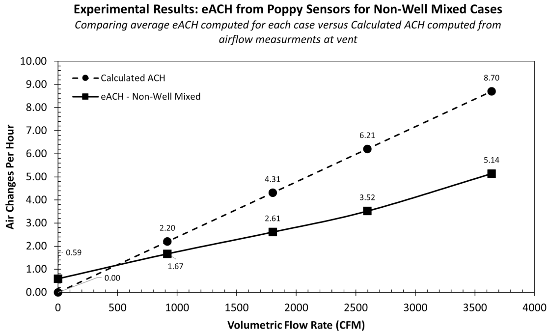
Figure 29. Calculated air change rate and average measured effective air change rates versus the volumetric flow rate for non-well mixed cases in the physical test space. As increasing rates of air are exchanged through the physical test space, the effective ACH increases but at a slower rate. A deviation as high as 43% is noted.
