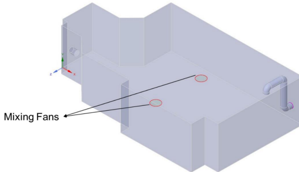
Figure 18. The geometric setup of the realistic case with one inlet pipe, one outlet pipe unit and two mixing fans placed inside the room. The airflow inside the room was designed to operate at 2000 CFM.
