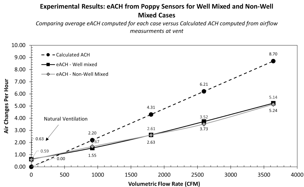
Figure 30. Calculated ACH & measured eACH versus the volumetric flow rate for well mixed and non-well mixed cases in the physical test space.
