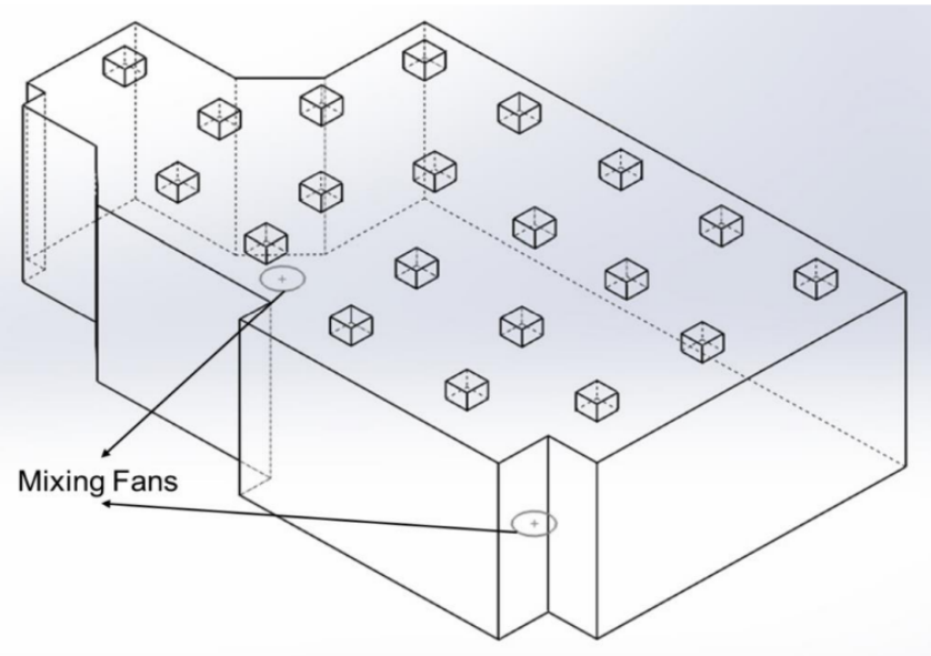
Figure 5. The geometric setup of the standard HVAC case with 10 supply units and 10 return units designed according to the ASHRAE and SMACNA Standards, with mixing fans placed inside the room.
