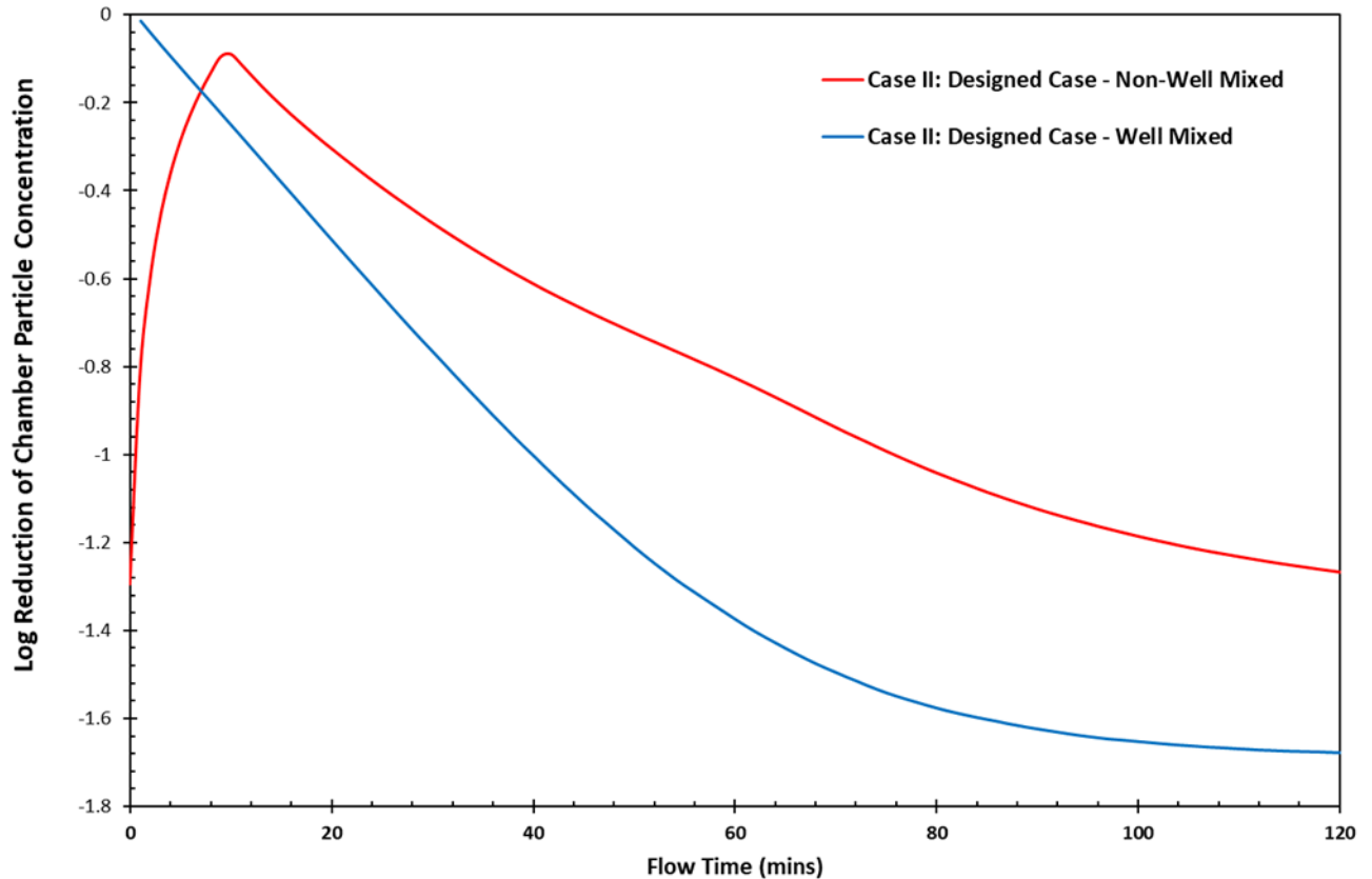
Figure 22. Total reduction of particles inside the realistic case test chamber with one inlet pipe and one outlet pipe, being operated to achieve a total room flow rate of 2000 CFM. The particles were released from the center of the room, releasing 1 million particles in 10 minutes, comparing the designed case with and without mixing fans.
