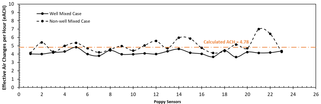
Figure 27. eACH captured by 23 sensor locations modeled in the virtual test space with a designed ventilation system for a well mixed and a non-well mixed case. The well mixed case had lower spatial variability than the non-well mixed case.
