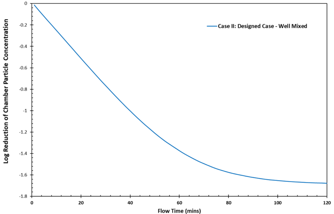
Figure 20. Total reduction of particles inside the realistic case test chamber with one inlet pipe, one outlet pipe and mixing fans placed inside the room. The particles were released from the center of the room, releasing 1 million particles in 10 minutes. The airflow inside the room was designed to operate at 2000 CFM.
