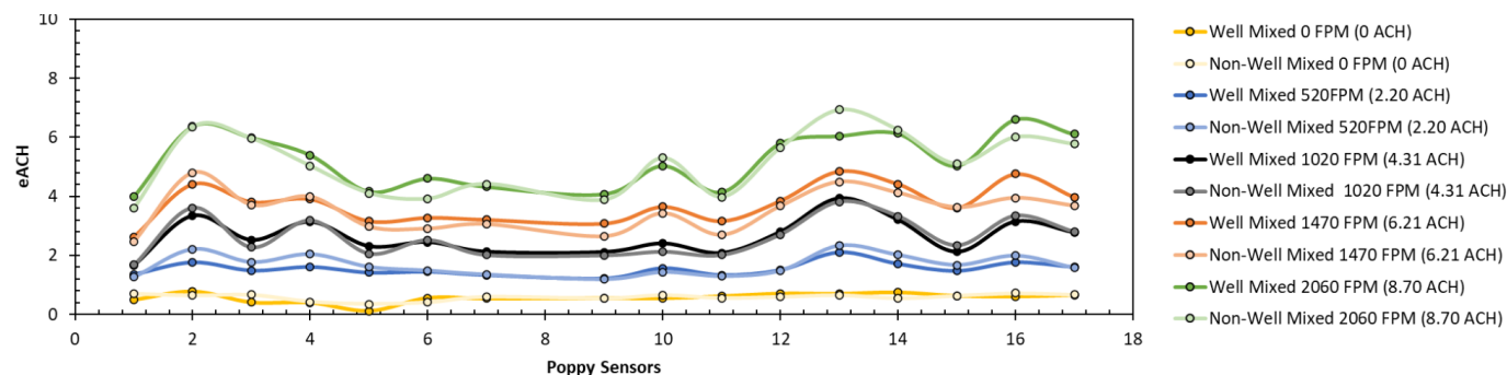
Figure 31. Positional spatial variation of eACH for a well mixed and a non-well mixed case for four different volumetric flow rates in the physical test space. Spatial variation is observed closer to the inlet, outlet, and walls.
