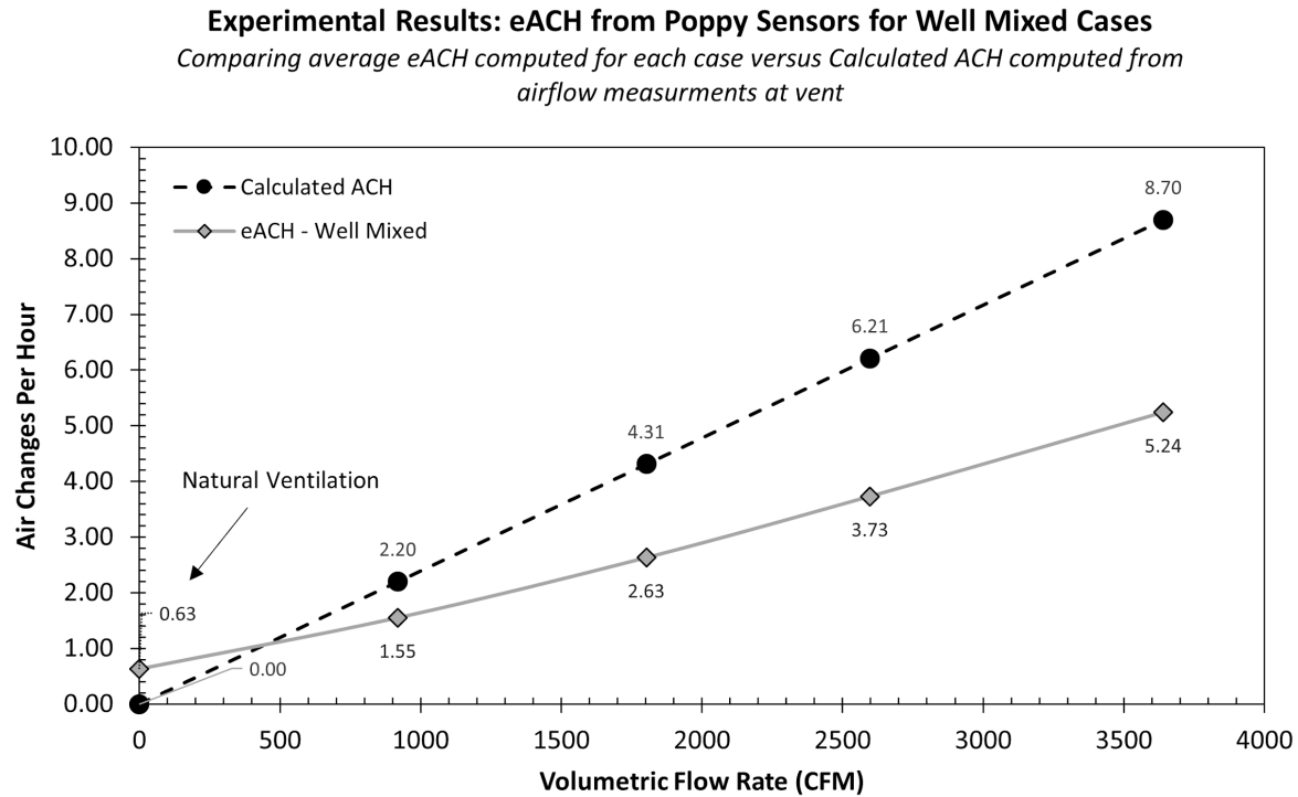
Figure 28. Calculated air change rate and measured effective air change rate versus the volumetric flow rate for well mixed cases in the physical test space. As increasing levels of air are exchanged through the test space, the effective ACH increases but at a slower rate. A deviation as high as 40% is noted.
