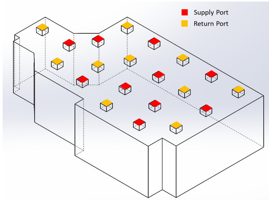
Figure 2. The geometric setup of the standard HVAC case with 10 supply units and 10 return units designed according to the ASHRAE and SMACNA Standards.
