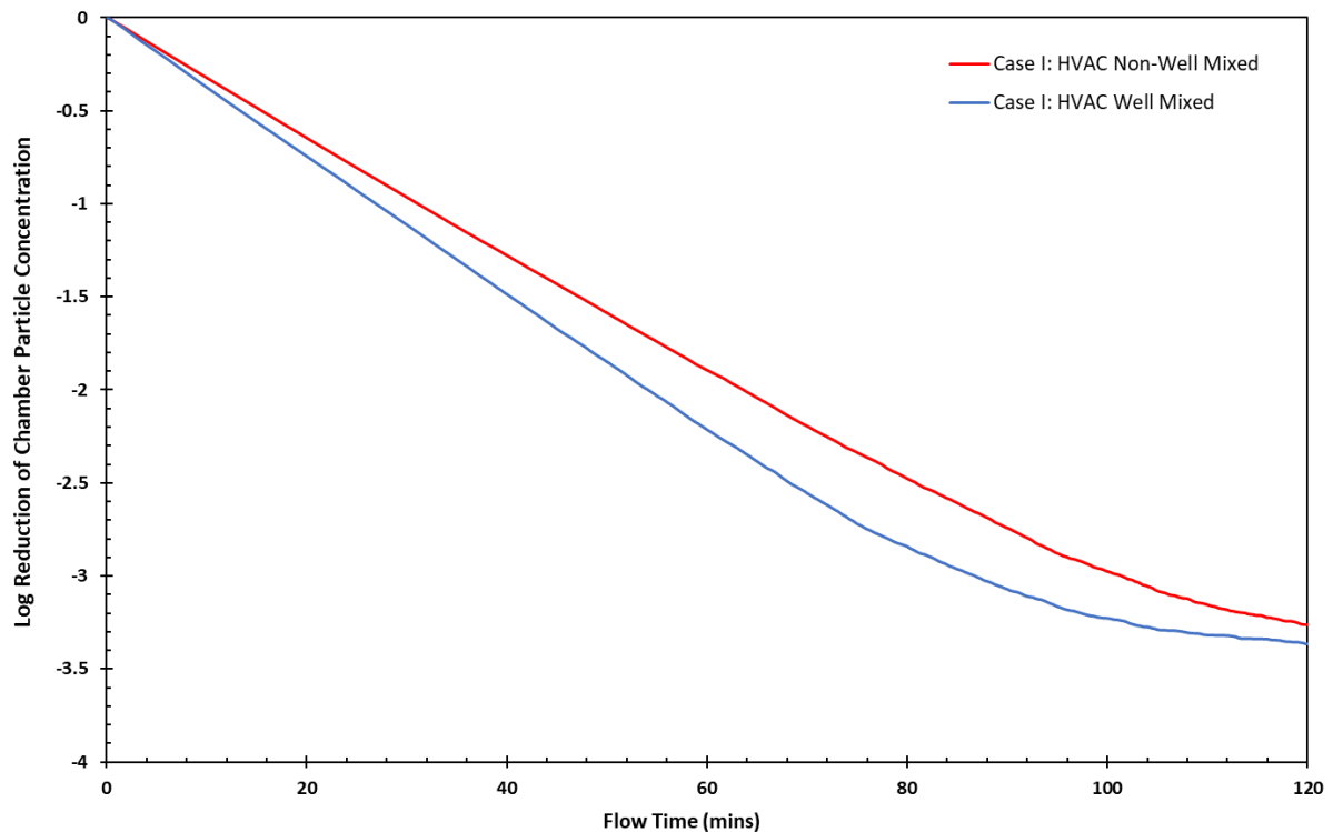
Figure 8. Total reduction of particles inside the virtual test chamber, with 10 supply vents and 10 return vents, being operated to achieve a total room flow rate of 2000 CFM; Comparing standard HVAC case without and with mixing fans
