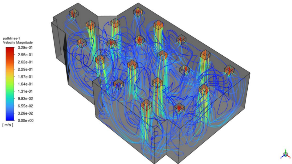
Figure 3. Flow inside the standard HVAC layout, numerically simulated chamber with 10 supply vents and 10 return vents, being operated to achieve a total room flow rate of 2000 CFM.
