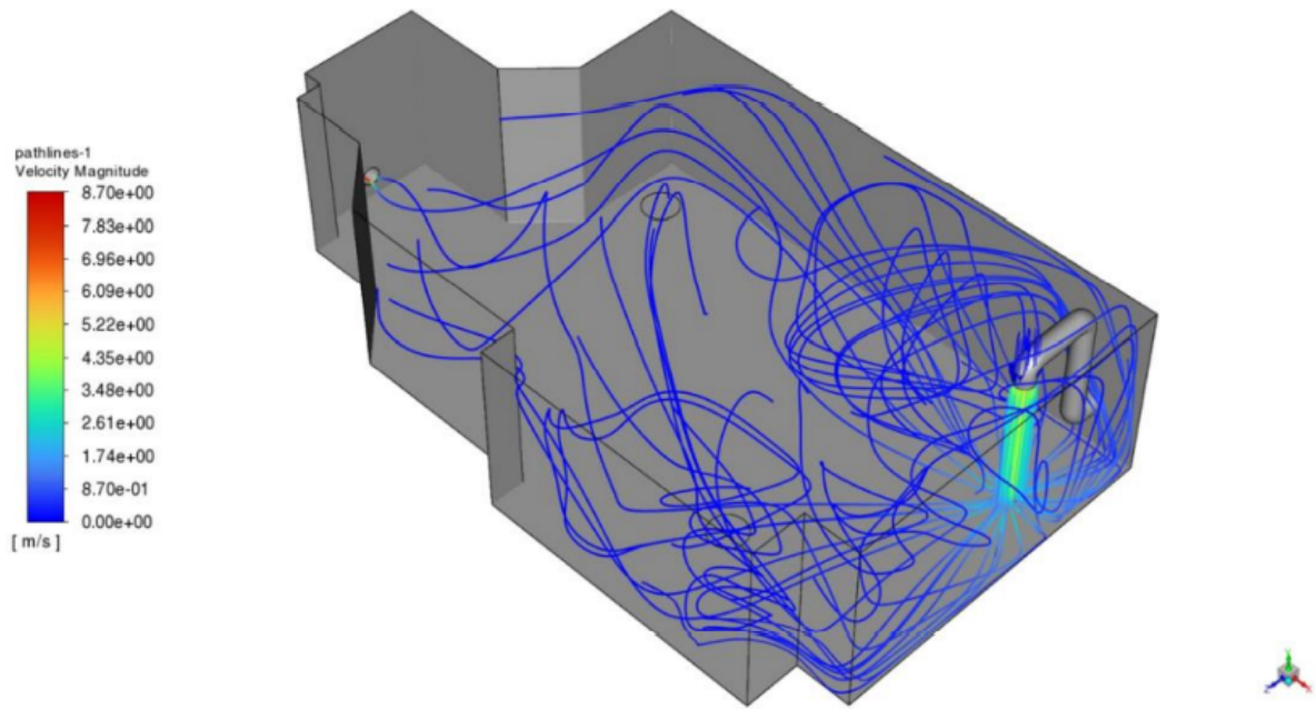
Figure 13. Flow inside the designed ventilation system, numerically simulated chamber with one inlet pipe and one outlet pipe unit, with mixing fans placed inside the room. The airflow inside the room was designed to operate at 2000 CFM.
