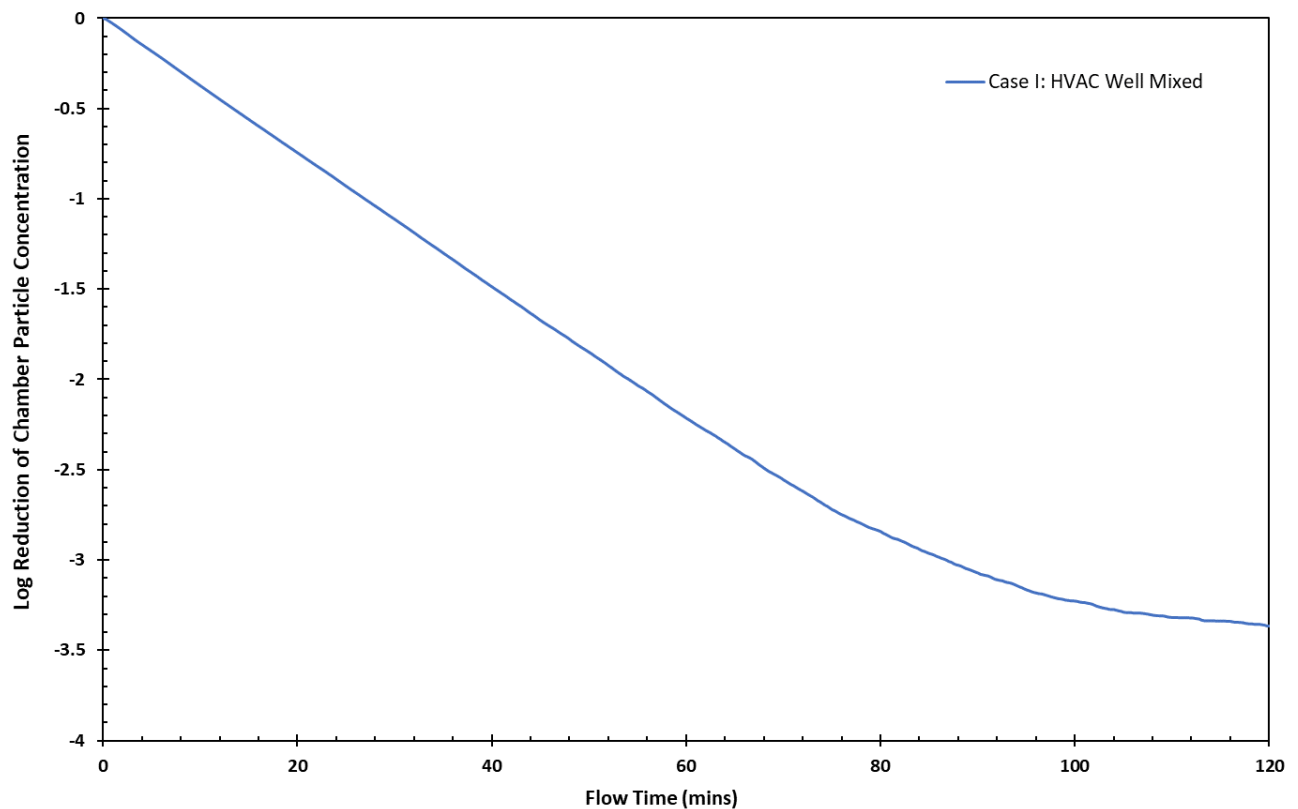
Figure 4. Total reduction of particles inside the standard HVAC test chamber, with 10 supply vents and 10 return vents, operated to achieve a total room flow rate of 2000 CFM.
