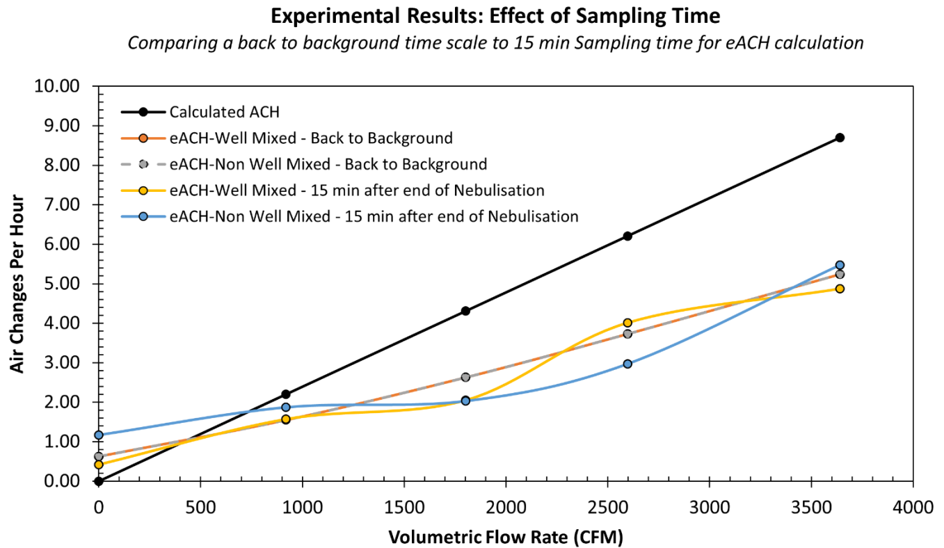
Figure 32. Effect of decay sampling time on the computation of eACH for all physical test cases.
