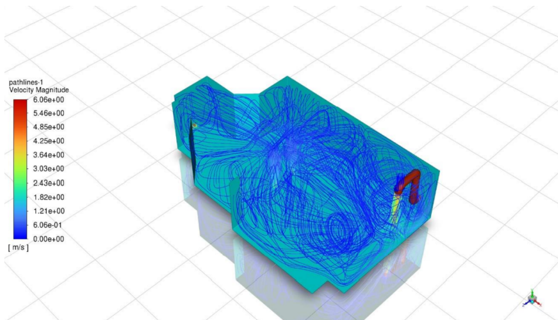
Figure 19. Flow inside the realistic case, numerically simulated chamber with one inlet pipe, one outlet pipe unit and with mixing fans placed inside the room. The airflow inside the room was designed to operate at 2000 CFM.
