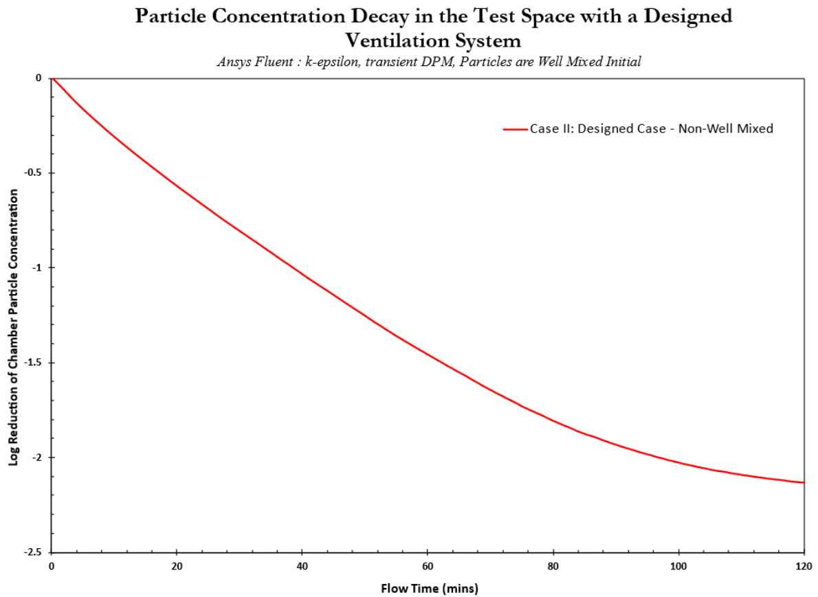
Figure 14. Total reduction of particles inside the designed ventilation system test chamber with one inlet pipe and one outlet pipe, with mixing fans placed inside the room. The airflow inside the room was designed to operate at 2000 CFM.
