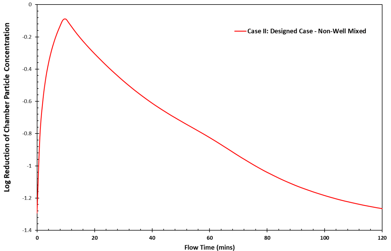
Figure 17. Total reduction of particles inside the test chamber with one inlet pipe and one outlet pipe unit placed inside the room. The particles were released from the center of the room, releasing 1 million particles in 10 minutes. The airflow inside the room was designed to operate at 2000 CFM.
