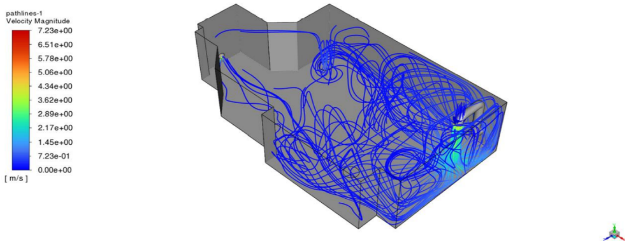
Figure 10. Flow inside the designed ventilation system, numerically simulated chamber with one air inlet and one air outlet inside the room. The airflow inside the room was designed to operate at 2000 CFM.
