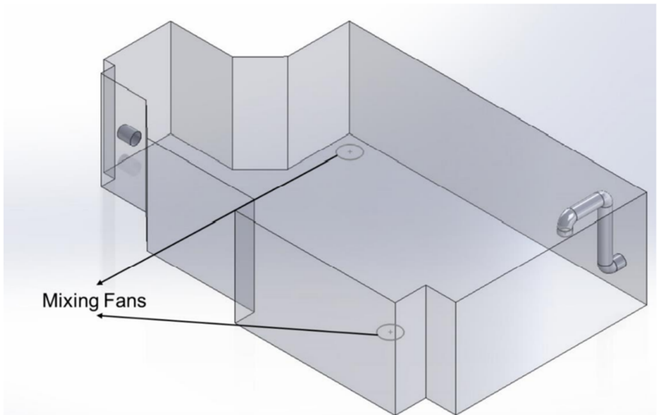
Figure 9. The geometric setup of the designed ventilation system case with one inlet pipe and one outlet pipe inside the room. The airflow inside the room was designed to operate at 2000 CFM.
