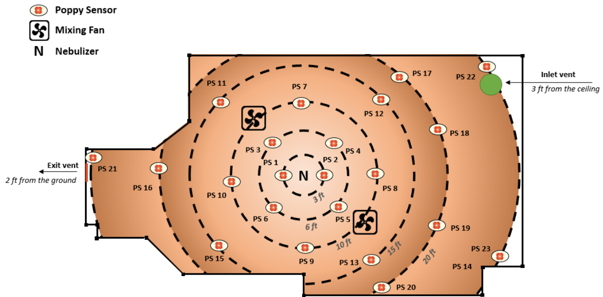
Figure 16. The geometric setup of the realistic ventilation case with one inlet pipe, one outlet pipe unit and two mixing fans placed inside the room. This is the extension to the case from the previous phase with 23 simulated Poppy Sensor devices to detect particles inside the chamber. The particles were modeled to release from the center of the room. The airflow inside the room was designed to operate at 2000 CFM.
