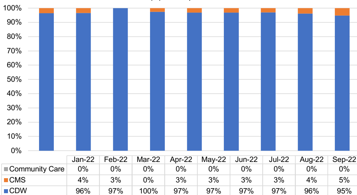
(B) Molnupiravir
