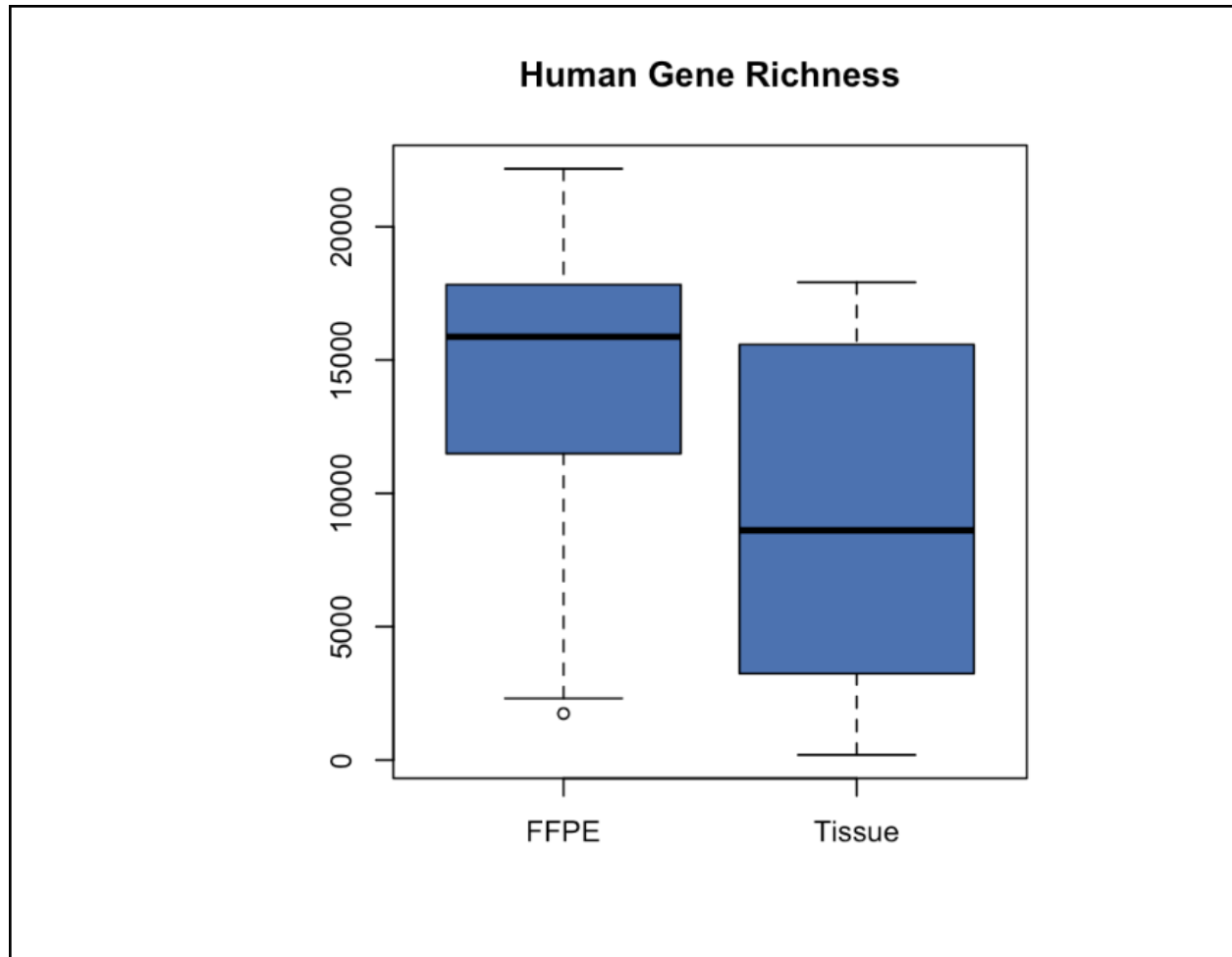
Figure 1: FFPE samples perform comparably or better to fresh tissue for basic sequencing metrics. FFPE samples detected a similar number of species (A), KOs (B), and had a similar %Microbial ESD (C) compared to fresh tissue ( p>0.05 ); FFPE samples detected more human genes (D) than the fresh tissue ( p=0.0099 ).
