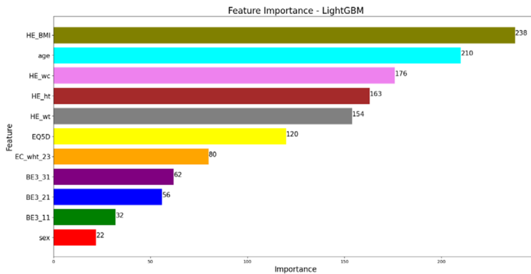
Figure 4. Feature importance of LightGBM model
