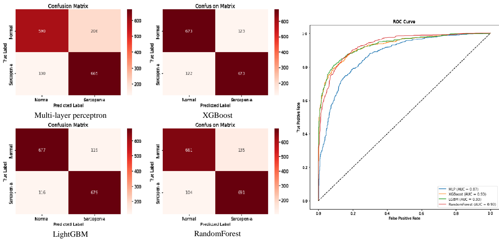
Figure 2. Confusion matrix and ROC-AUC curve of sarcopenia prediction model
