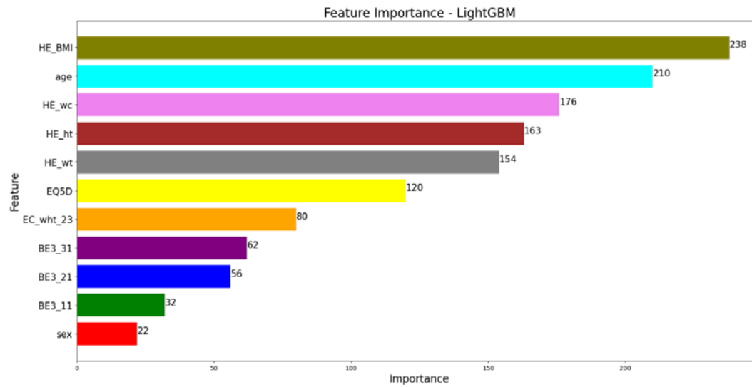
Figure 4. Feature importance of LightGBM model
