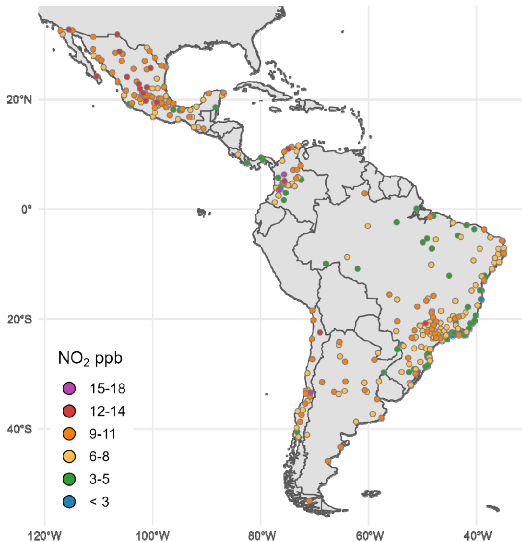
Figure 1. Location of study cities (N=326) and city-level population-weighted annual concentration of ambient NO 2 in 2019. The WHO guideline for annual NO 2 is 10 µg/m 3 (≈ 5.3 ppb) and all neighborhoods that exceed this guideline are represented by yellow, orange, red, or purple.
