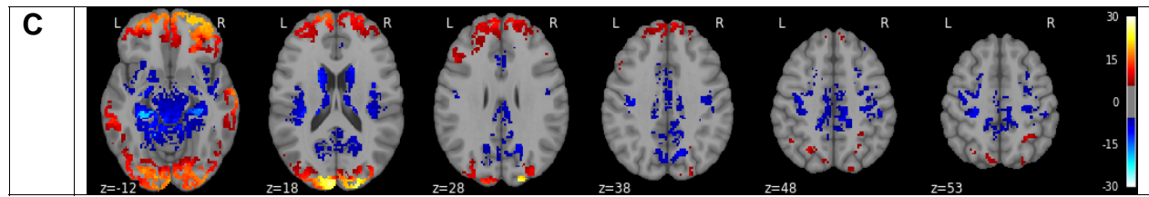
Figure 3: Regional BEN changes induced by the relational task. A) resting BEN vs BEN of the task relational; B) control BEN (BEN of the task control condition) vs BEN of the task relational condition; C) resting BEN minus control BEN. Hot and blue color mean higher and lower BEN at the resting state, respectively. Color bars indicate the display window for the t-value of the paired-t test.
