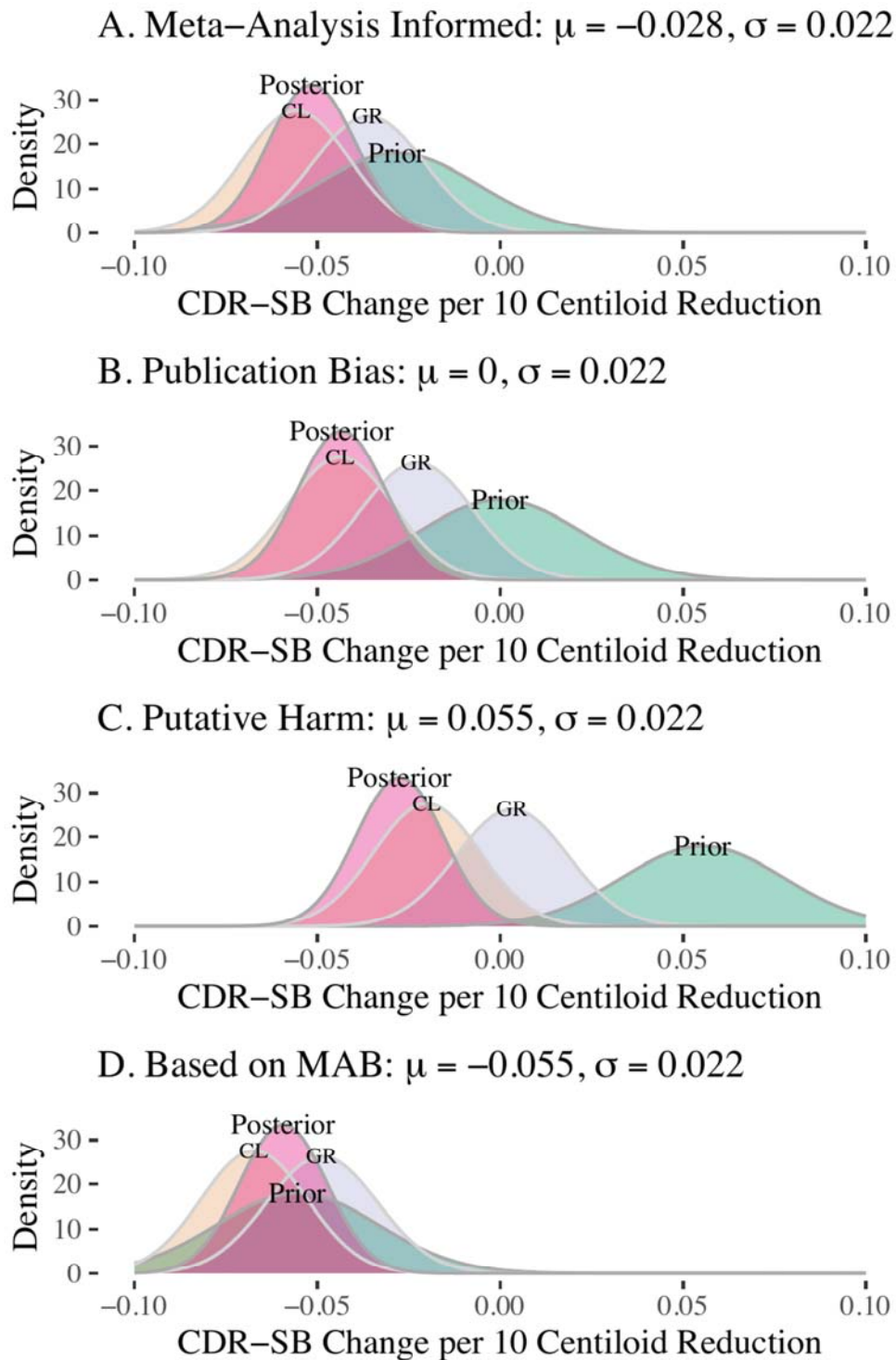
Figure 1: Prior intervals and posterior distributions for the effect of a 10 centiloid reduction on CDR-SB for the four main starting positions. Panels A-D correspond to the four starting positions outlined in Tables 1 and 2. Each panel shows the prior, a posterior updated with just
