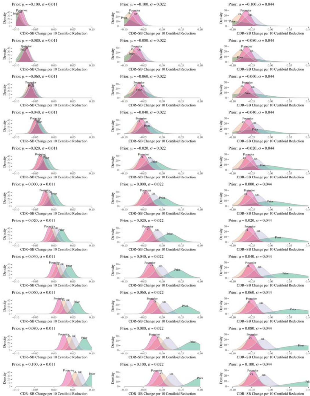
Figure S1: Prior and posterior distributions for the effect a 10 centiloid reduction on CDR-SB change for narrow, moderate, and wide starting prior distributions. Mean ( \mu ) and standard deviation ( \sigma ) are given in the panel labels.
