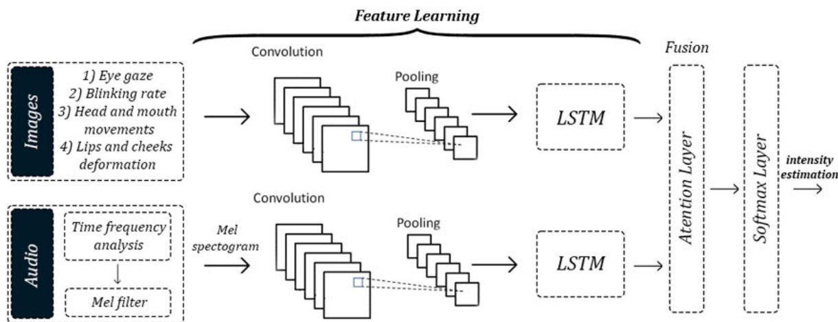
Figure 3: Neural network architecture of the proposed CNN/LSTM multimodal network.
