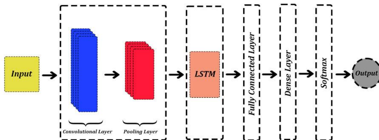
Figure 2: Neural network architecture of the proposed single modality CNN/LSTM network.
