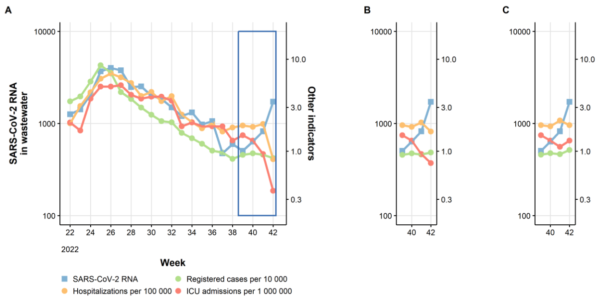
236 Figure 3. Timeliness of gathering complete results by different surveillance systems over a defined 237 week: A) WS data updated on Mondays (blue), B) hospitalizations (yellow) and registered cases 238 (green) data updated on Wednesdays and C) ICU admissions (red) data updated on Fridays.
