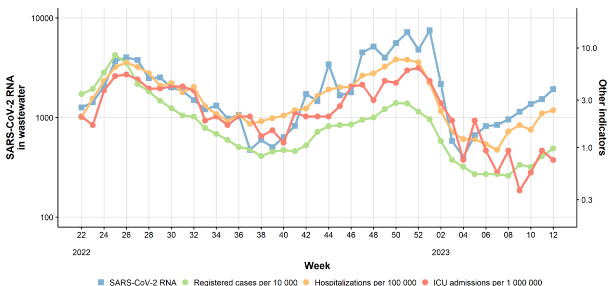
196 Figure 1. Weekly level of SARS-CoV-2 RNA detected in wastewater in Norway (blue line), compared 197 with clinical indicators for COVID-19. SARS-CoV-2 RNA levels in wastewater are population-weighted 198 and PMMoV-normalized. Note: the wastewater data are based on results of samples taken at 199 selected locations, while the clinical indicators are based on data from national registries (Beredt- 200 C19).
