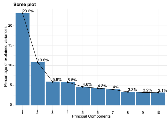
B Principal component analysis: Scree plot of eigenvalues of principal components
