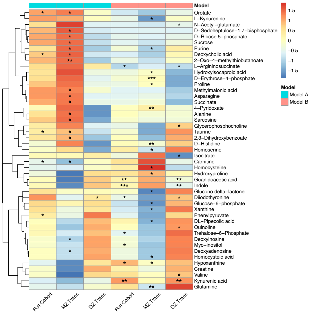
A Heatmap of estimate ( \beta ) values from GEE model for metabolites and autism diagnosis
