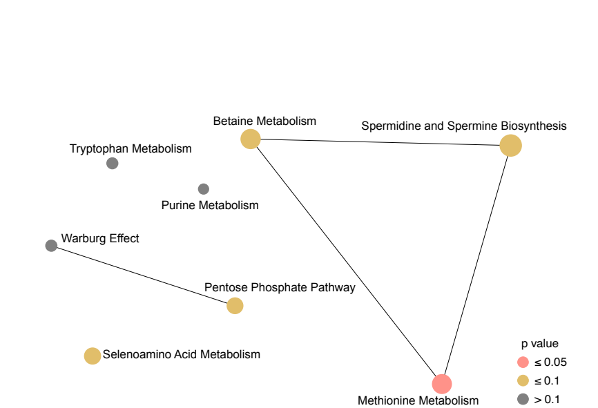
D Full Cohort: Interaction network for enriched pathways based on autistic traits and GEE Model B.
