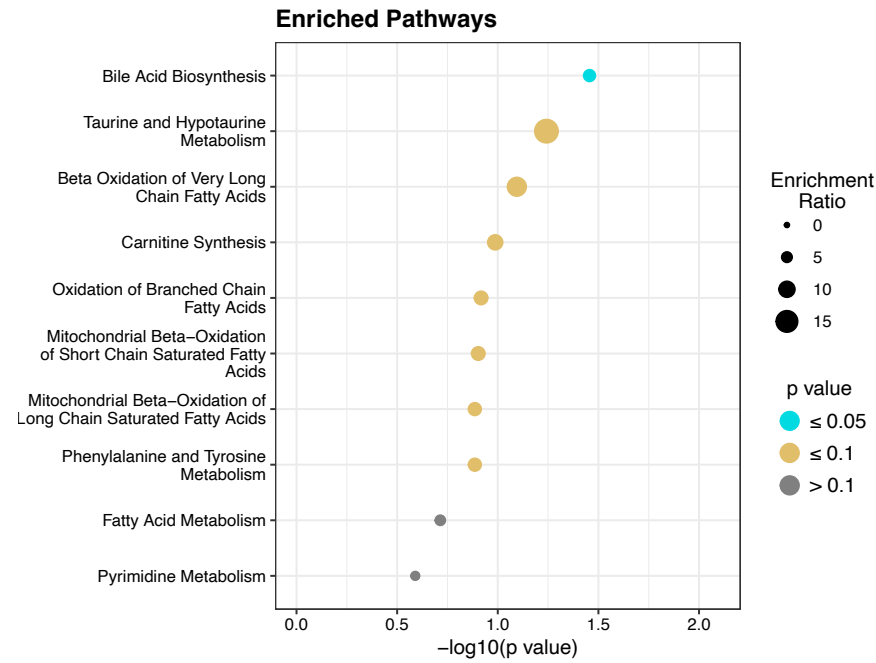
A Full Cohort: Enrichment dot-plot for top 10 enriched pathways based on autism diagnosis and GEE Model A.
