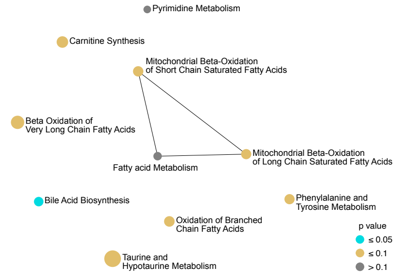
B Full Cohort: Interaction network for enriched pathways based on autism diagnosis and GEE Model A.
