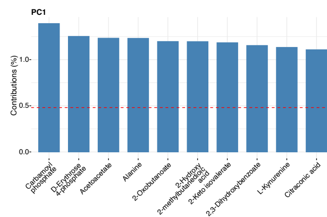
C Principal component analysis: Metabolites contributing to Principal Component 1
