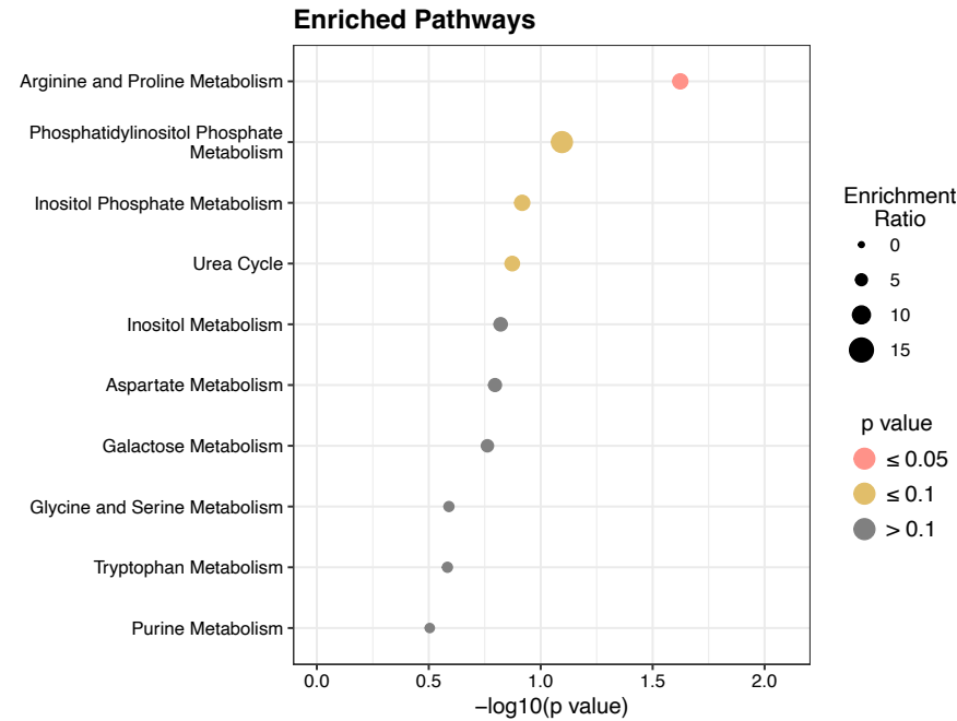
C Full Cohort: Enrichment dot-plot for top 10 enriched pathways based on autism diagnosis and GEE Model B.
