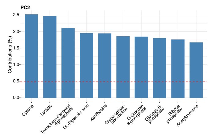
D Principal component analysis: Metabolites contributing to Principal Component 2
