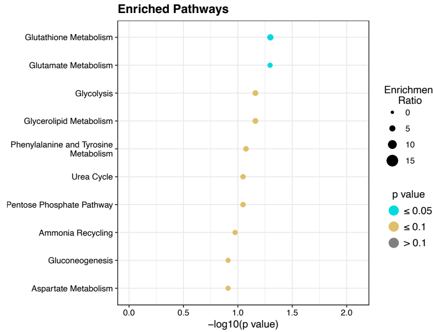
A Full Cohort: Enrichment dot-plot for top 10 enriched pathways based on autistic traits and GEE Model A.
