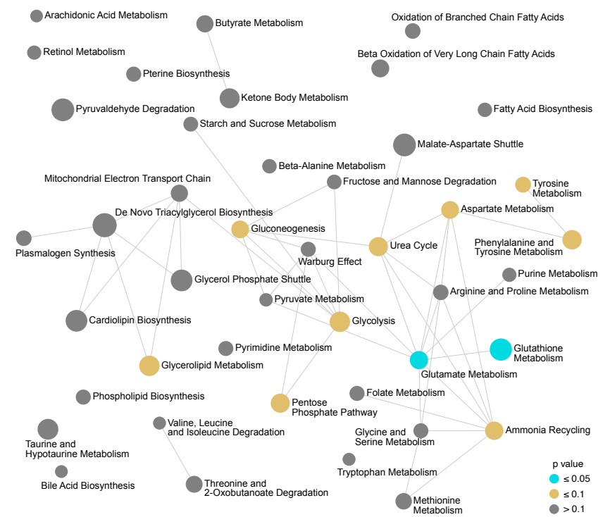
D Full Cohort: Interaction network for enriched pathways based on autistic traits and GEE Model B.
