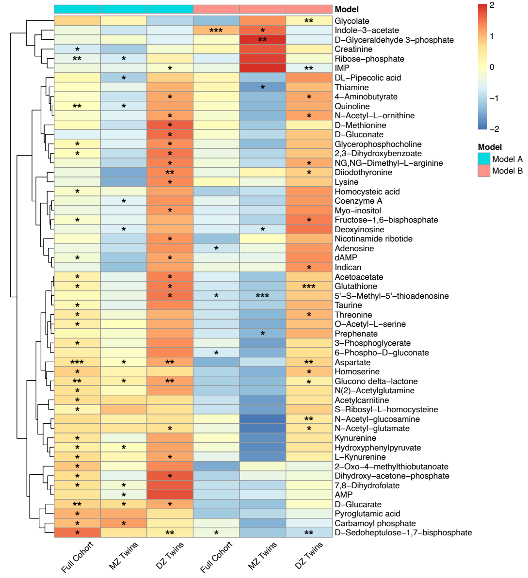
B Heatmap of estimate ( \beta ) values from GEE model for metabolites and autistic traits
