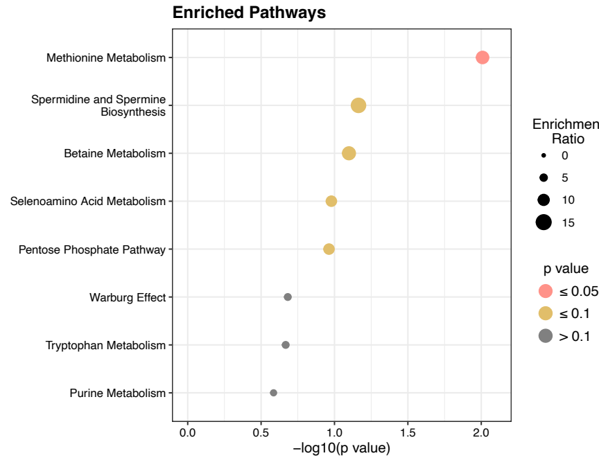
C Full Cohort: Enrichment dot-plot for top 10 enriched pathways based on autistic traits and GEE Model B.
