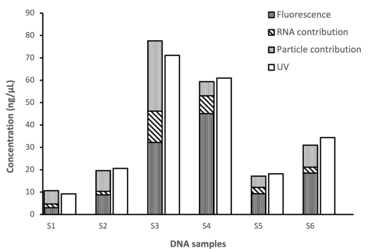
Fig 6. Contribution of magnetic particles and RNA to DNA concentration measurements by UV absorbance spectrophotometry.
