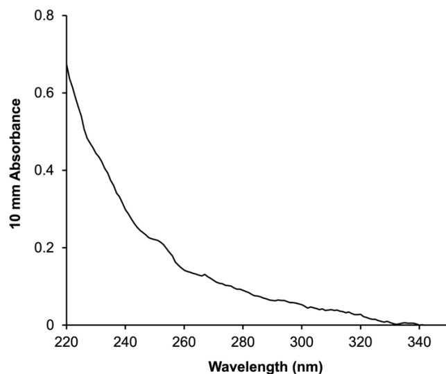
Fig 1. Absorbance spectrum of the magnetic particles.
