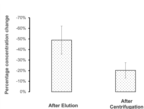
Fig 5. Difference between the DNA concentration measured by UV spectrophotometry and fluorescence. DNA concentration was measured after elution from the extraction column, both by UV spectrophotometry and fluorescence. Residual magnetic particles were then removed from the DNA samples by centrifugation, before DNA concentration was measured again. The difference between the concentration measured by UV spectrophotometry and fluorescence is displayed as a percentage change. Bars represents standard deviation.
