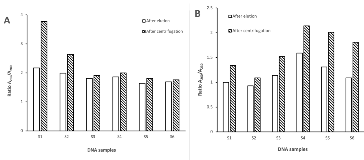
Fig 4. Absorbance ratios before and after particle removal. The absorbance ratios A_{260}/A_{280} (A) and A_{260}/A_{230} (B) of the DNA samples were measured before and after magnetic particles removal by centrifugation.
