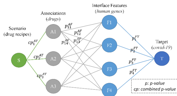
Figure 5: The general structure of the native ML model to suggest an effective drug combination in the treatment of disease using human genes as interface features
