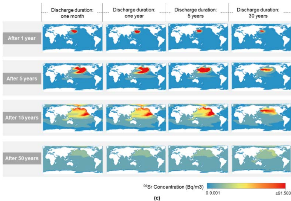
Fig.1 Spatial distribution of activity concentration by radionuclides under different discharge scenarios
