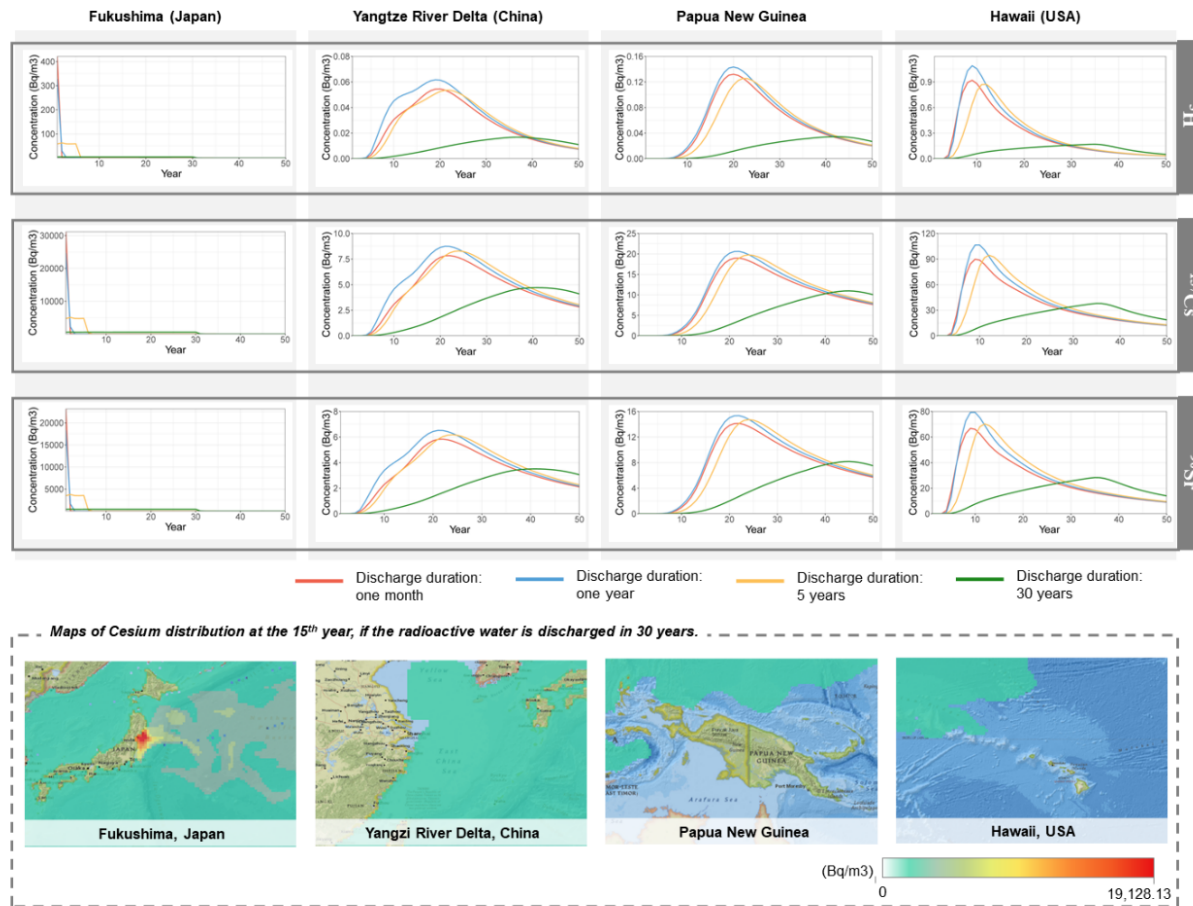
Fig.3 Activity concentrations of sea surface water in Fukushima (Japan), Yangtze River Delta (China), Papua New Guinea, and Hawaii (USA) by radionuclides and release scenarios.
