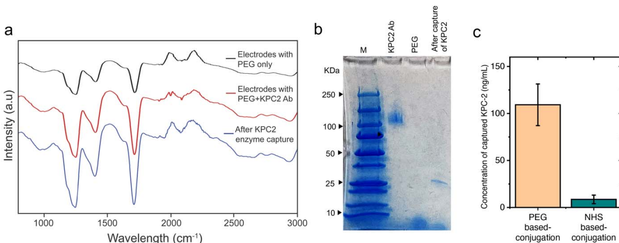
Figure 4. Characterization of antibody-modified Au-SPEs and KPC2 enzyme capture efficiency. (a) FTIR analysis of the modified (in red) and unmodified electrodes (in black), and modified electrodes after enzyme capture (in blue) (protein specific range at what wavenumber?)
