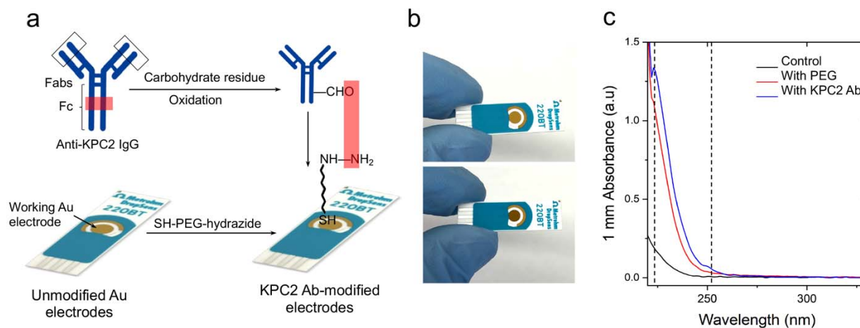
Figure 1. PEG-mediated conjugation of IgG antibodies to the surface of screen-printed gold electrodes. (a) Schematic presentation of the protocol for chemical modification of Au-SPE with SH-PEG-hydrazide followed by coupling with antibody. (b) Digital images of unmodified (top) and modified Au-SPE (bottom), showing a change in color of the surface post-modification. (c) UV-Vis spectrum of control Au-SPE (without any treatment; black line), PEGylated Au-SPE (red line) and antibody-coupled Au-SPE (blue line). The surface of Au-SPEs was digested with TCEP, and the eluted solution was tested using a NanoDrop spectrophotometer to measure the absorbance.
