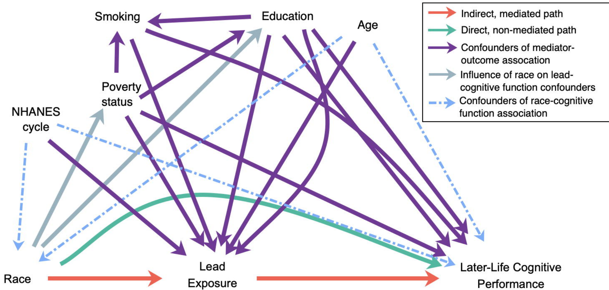
Figure 1. Directed acyclic graph (DAG) causal diagram representing hypothesized causal relationships among mediators and confounders of the association between marker of racism/racialized experience (Black vs White), lead exposure, and later-life cognitive function.
