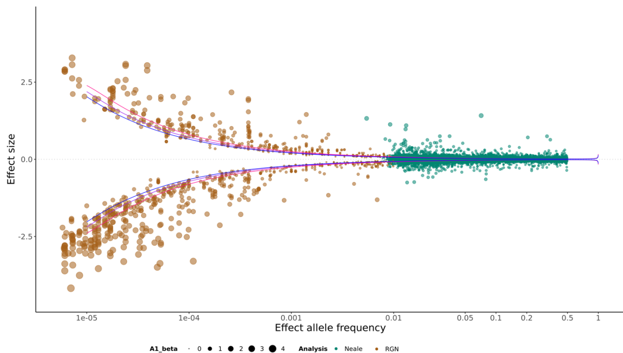
164 165 Figure 1. Distribution of allele frequencies and effect sizes for genetic associations across 129 166 continuous traits from the UK Biobank. Power curves for statistical power of 0.5 (blue), 0.7 (purple) 167 and 0.9 (pink) were constructed for the median GWAS sample size (N=351,550).
