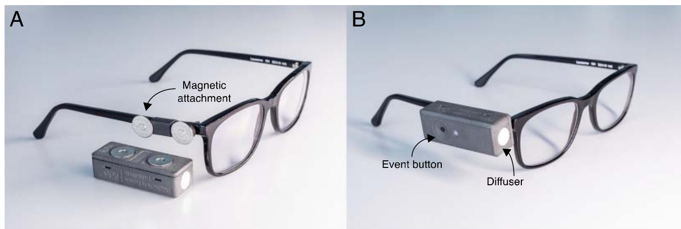
302 Figure 1: Wearable corneal-plane \alpha -opic light logger. A Light logger unattached to spectacle frame, 303 highlighting magnets for secure attachment. B Light logger attached to spectacle frames, highlighting 304 diffuser and event button for logging user-defined events. Photos by Licht@hslu.
