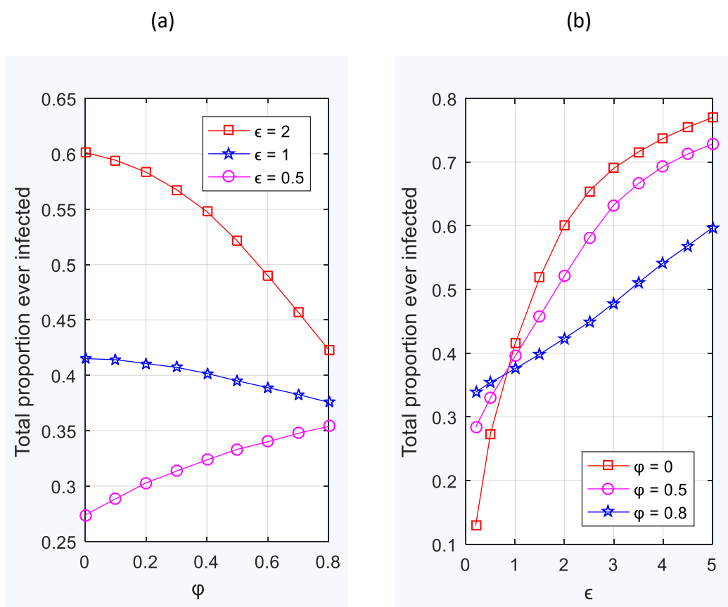
Fig 9 .1. Plot of total proportion ever infected at the end of 90 days, for initial condition I(0) = 1, C(0) = 1 and (a) Varying \varphi for \epsilon = 0.5, 1, 2 (b) Varying \epsilon for \varphi = 0, 0.5, 0.8
