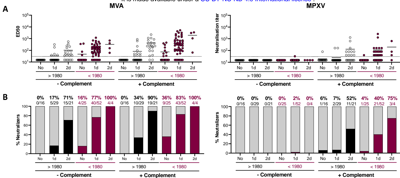
Fig. 3. Neutralizing antibodies induced by IMVANEX vaccination
