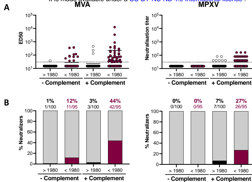
Fig. 1. Basal levels of neutralizing antibodies in unvaccinated and uninfected individuals
