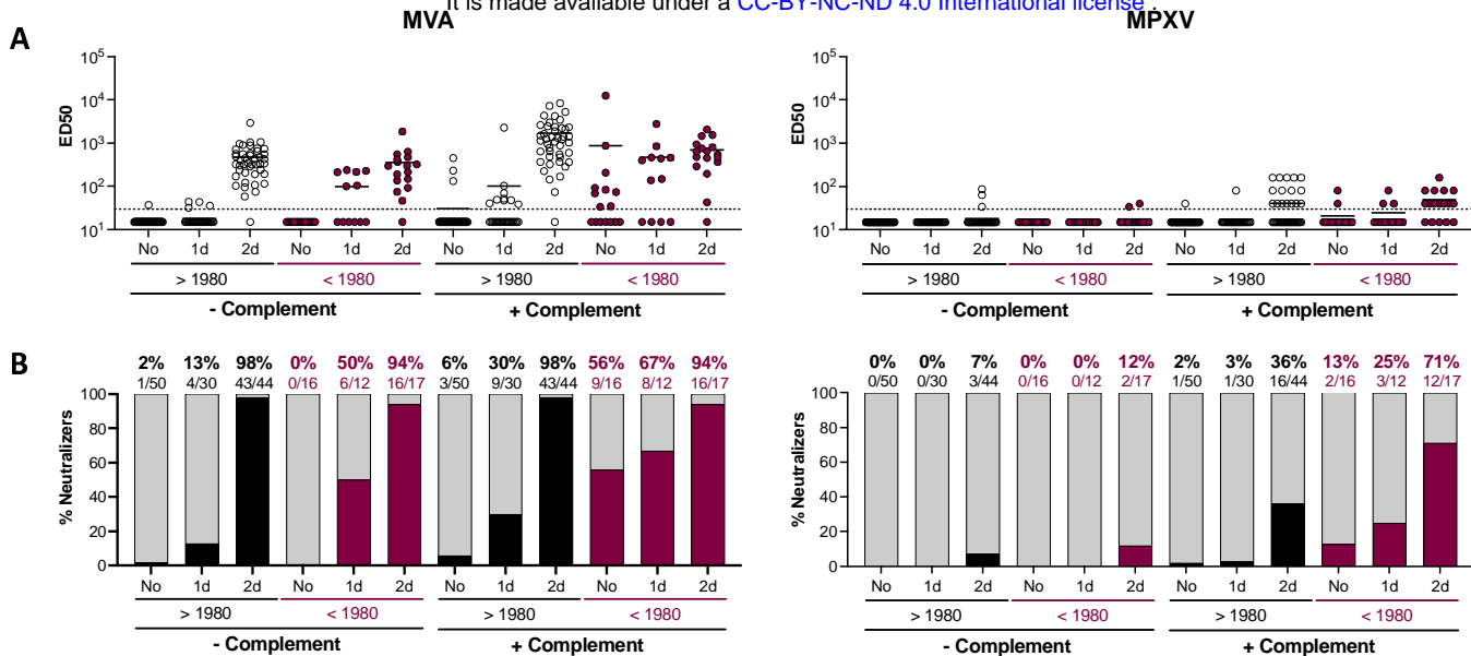
Fig. 4. Neutralizing antibodies induced by an experimental MVA-HIV vaccine
