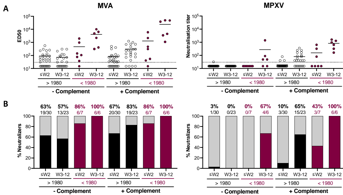
Fig. 2. Neutralizing antibodies induced by MPXV infection
