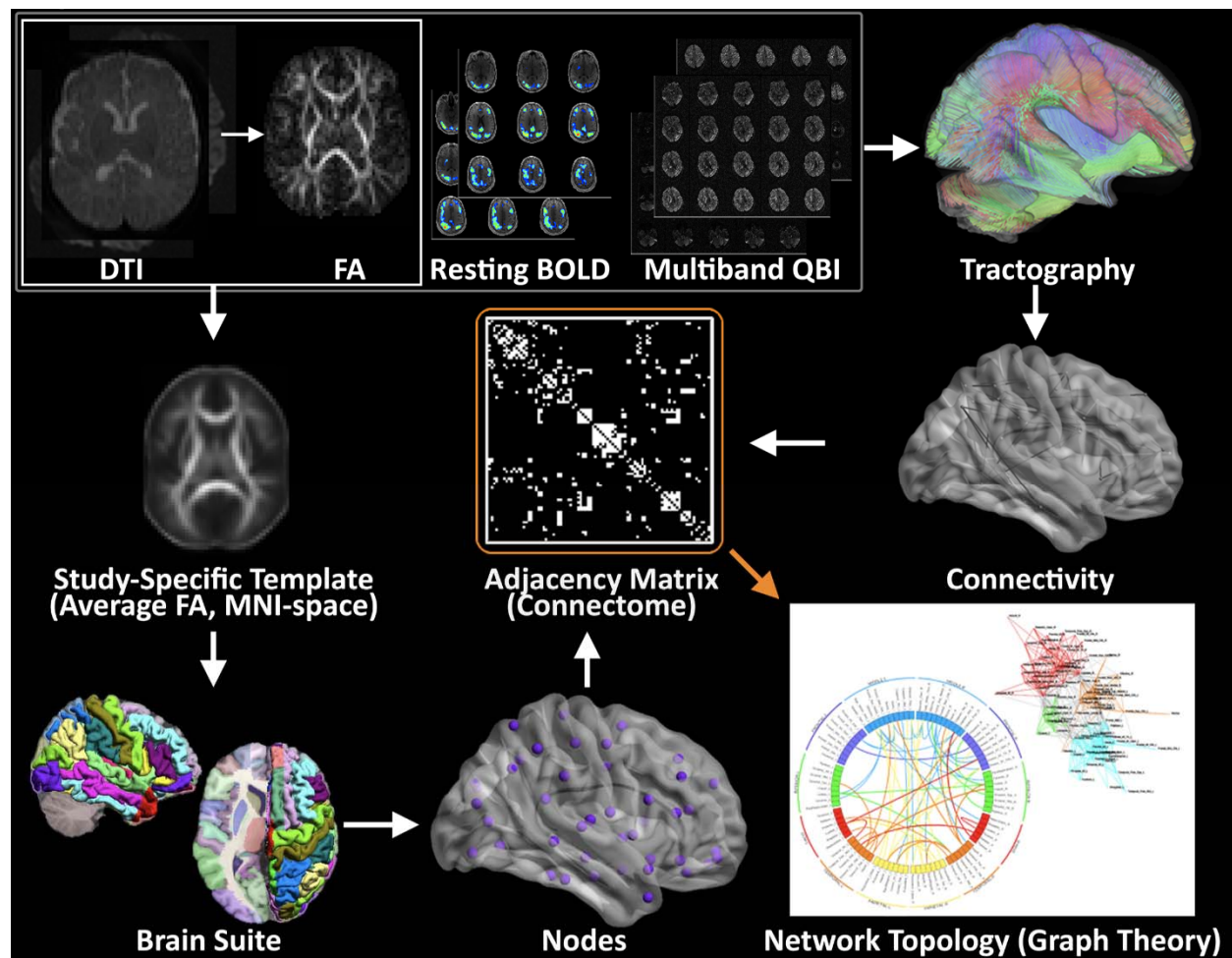
Figure 2: Methodology for Structural and Functional Network Topology Analysis.
