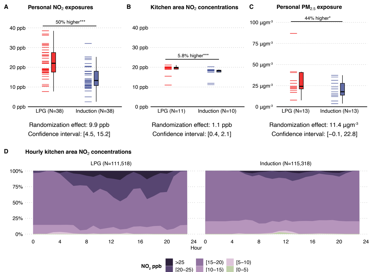
Figure 1: Personal and kitchen area air pollution concentrations when participants were instructed to use their LPG or induction stove exclusively and effect of randomization on pollution. In panels A–C, percent differences in means are estimated as based on the induction group average and estimated effect of randomization from the intention-to-treat analysis, which is noted below each panel along with the 95% confidence interval. Stars indicate statistical significance were P < 0.10 = * , P < 0.05 = ** , P < 0.01 = *** .
