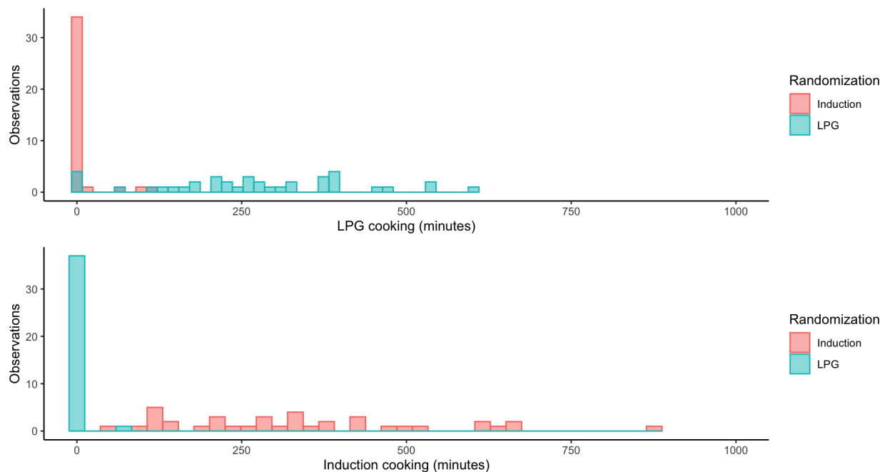
Figure S2: Minutes of detected LPG and induction stove use by randomization. In total, we observed deviations from assigned stove use during 4.4% of total cooking time when LPG and induction stove use were measured (272 out of 6243 minutes across 15 monitoring sessions).
