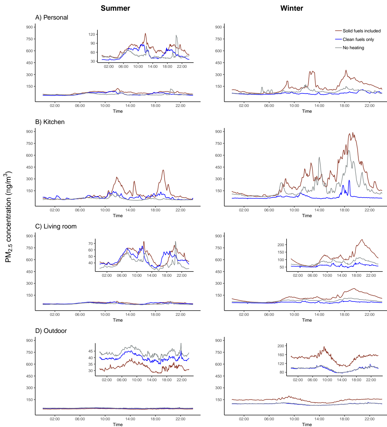
1 Figure 3. 24-hour average time-series plots for PM 2.5 concentrations (µg/m 3 ) recorded in the personal, kitchen, living room, and community monitors by season and primary heating fuel combinations 2
