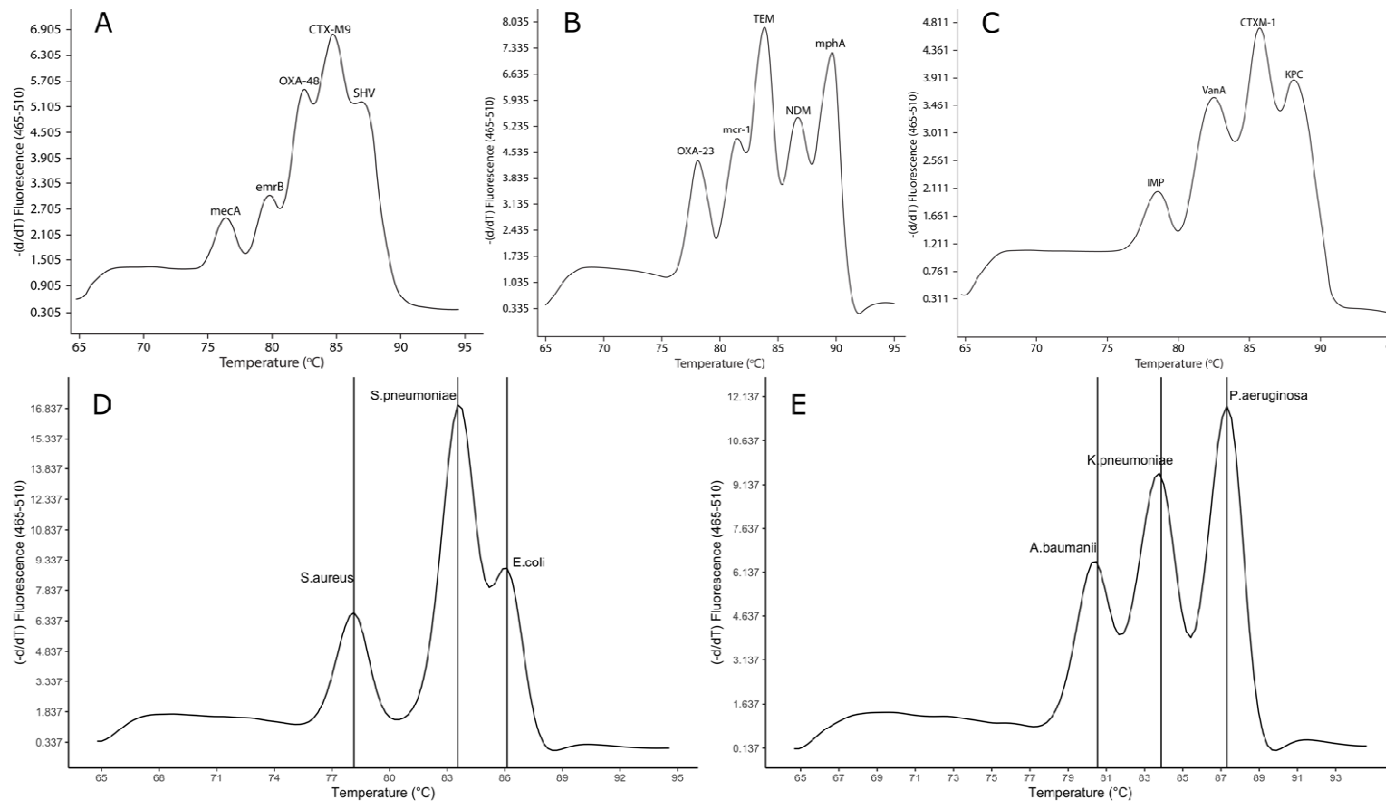
Figure 1. Melting curve analysis showing the melting temperature peaks ( T_m ) of 14 AMR genes (A, B, C) and 6 bacterial pathogens (D, E) and negative control (NTC) in 5 multiplex PCRs.
