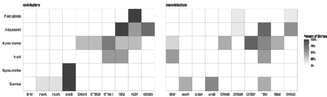
Figure 5. The distribution of predicted AMR genes in co-infections
