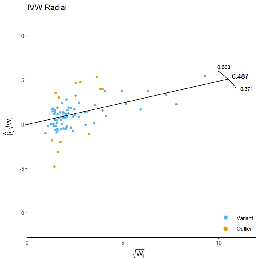
Fig 2. A scatter plot showing a radial IVW estimate using data from Do et al. Here the x-axis represents the square root of the weight applied to each SNP, while the y-axis shows the product of the ratio estimate and square root of the weight given to each SNP. Outliers are identified using Cochran’s Q-statistic and a p-value threshold of 0.05/number of SNPs has been used to correct for multiple testing.
