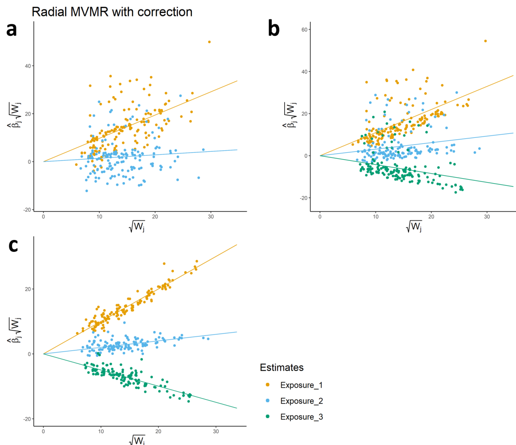
Fig 6. Panel showing radial MVMR plots corresponding to each of the simulated analyses presented in Table 1. Fig 6a represents the two-exposure model, while Fig 6b includes all measured exposures. Fig 6c, shows a plot generated after pruning pleiotropic SNPs identified in Fig 5.
