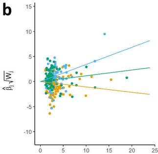
Radial MVMR with correction
