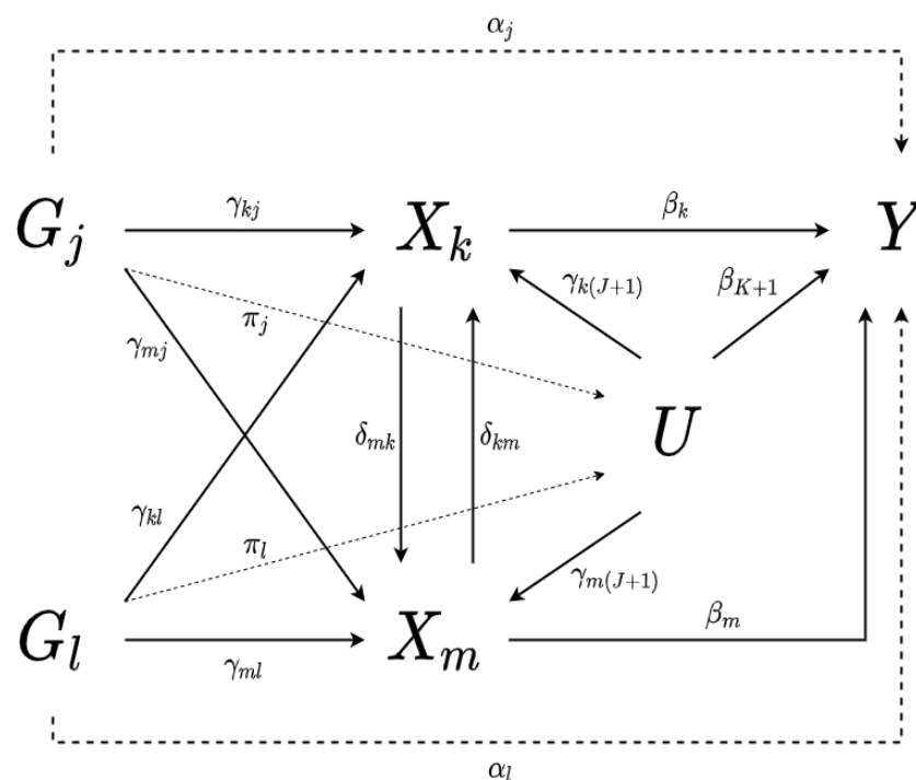
Fig 3. A DAG illustrating associations described in equations 1-2 and 9-10 for an arbitrary number of SNPs and exposures. Dashed lines represent associations which would violate assumptions MVMR2-3.
