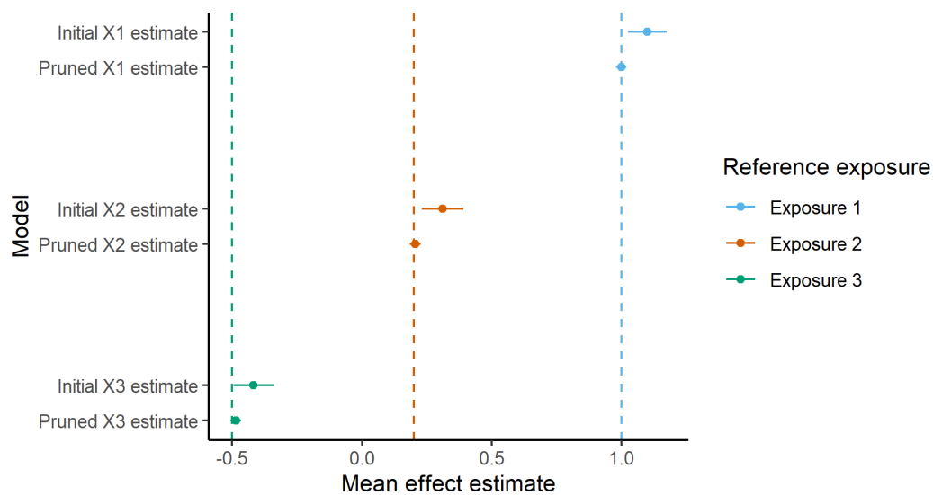
Fig 7. Forest plot showing mean effect estimates and 95% confidence intervals for the effect of exposures X_1 , X_2 , and X_3 following simulation 2. Vertical dashed lines depict defined true effects, coloured by exposure. Initial estimates indicate RMVMR estimates obtained prior to outlier pruning.
