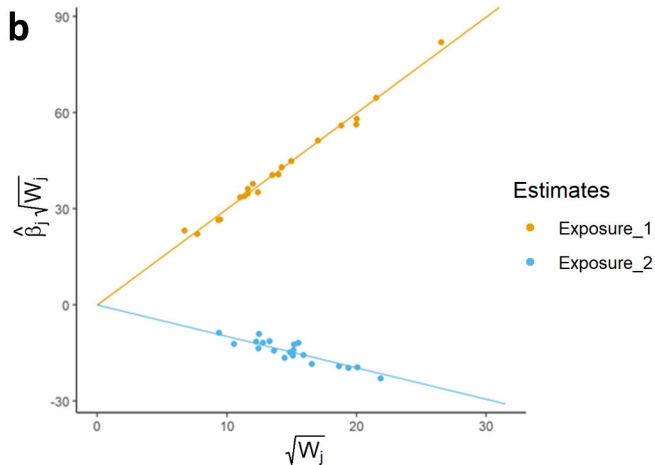
Radial MVMR with correction
