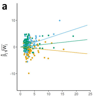
Radial MVMR without correction
