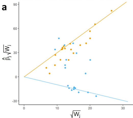
Radial MVMR without correction
