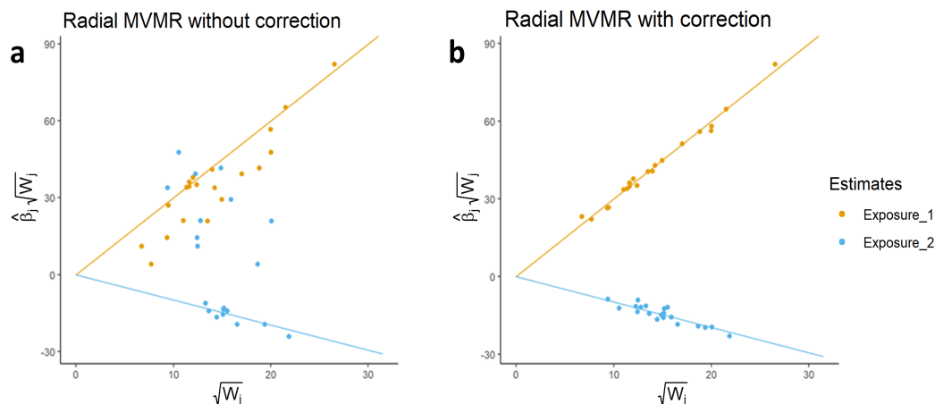
Fig 4. A pair of RMVMR plots using two exposures presented for illustration. In this case, both exposures have a non-zero effect on the outcome, and 10 instruments are associated with both exposures simultaneously. Fig 4a uses ratio estimates prior to adjusting for the additional exposure, resulting in substantial observed heterogeneity. Fig 4b shows a substantial reduction in observed heterogeneity when adjusting for the additional exposure.
