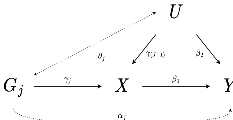
Fig 1. Directed acyclic graph (DAG) illustrating the assumptions of MR.
