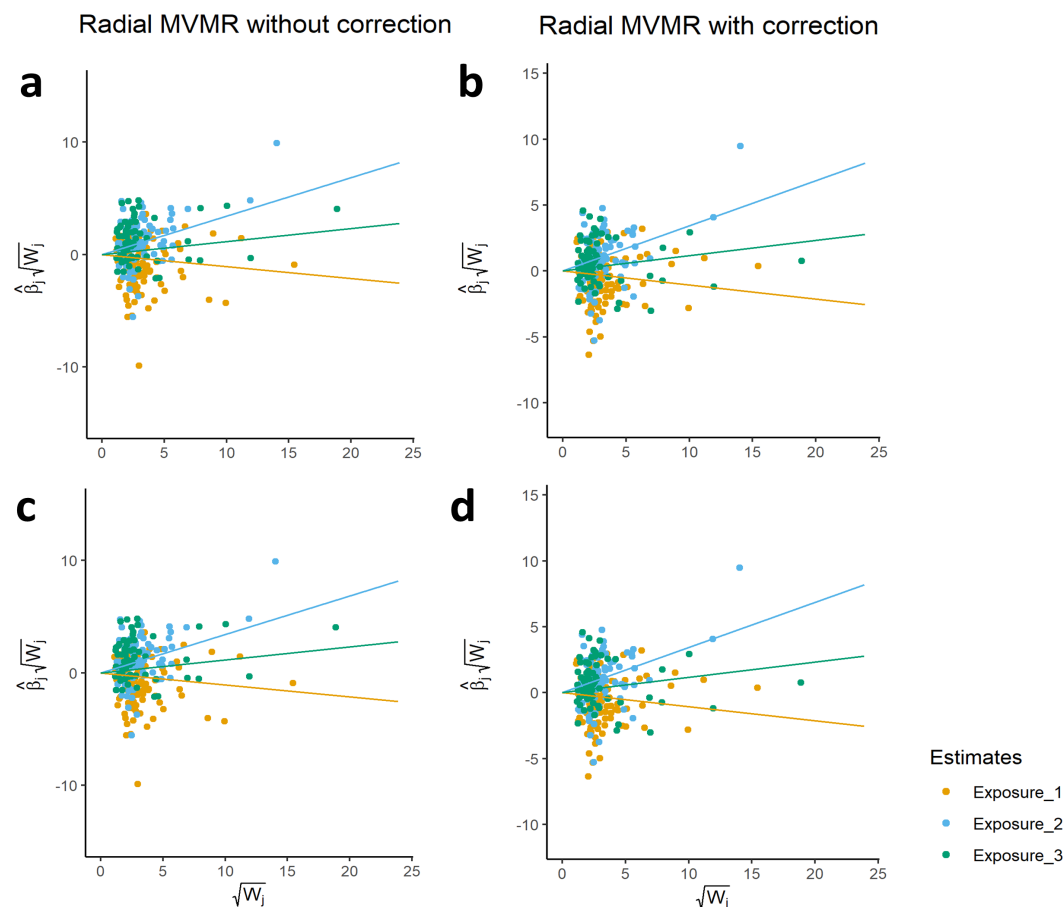
Fig 8. Panel showing RMVMR plots for applied analysis using HDL, LDL, and triglycerides. Observations correspond to ratio estimates and weightings with respect to each exposure. Regression lines represent MVMR causal effect estimates coloured by exposure. Fig 8a-8b correspond to the radial MVMR estimates prior to performing heterogeneity pruning, while Fig 8c-8d are constructed using heterogeneity pruned summary data.
