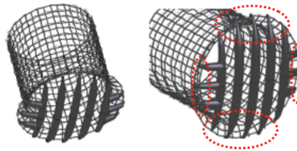
Figure 8: New deflector design. Lateral struts added are circled in red.
