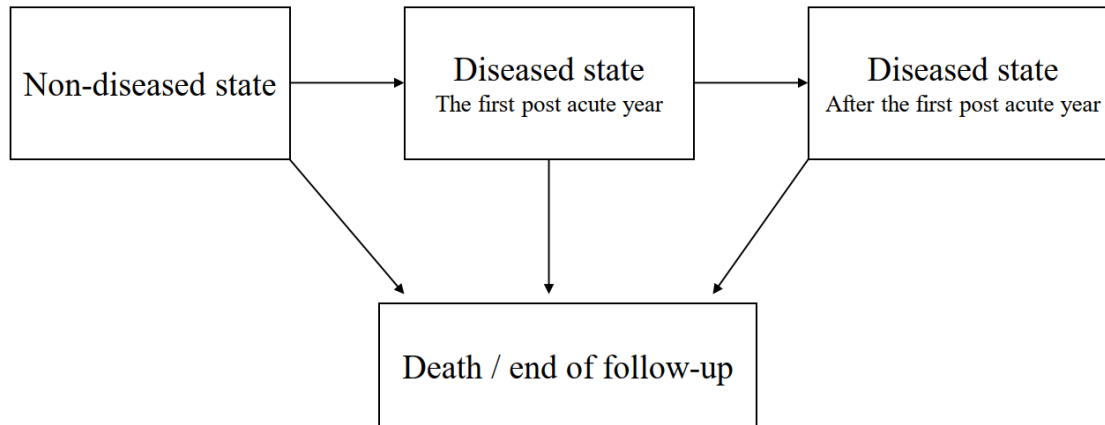
Figure 1. An extension of the illness–death model used in the analysis.
