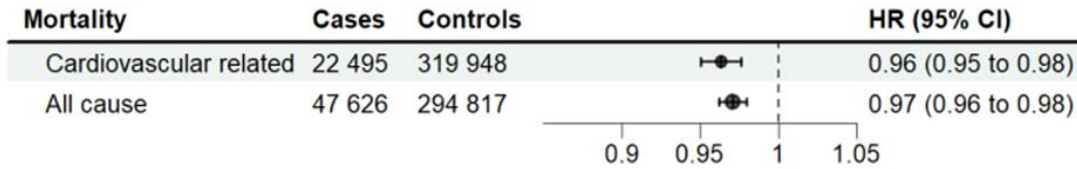
Figure 6. PRS HGS as a predictor of mortality. Multivariable Cox regression analysis. Adjusted for sex, collection year, genotyping batch, and ten principal genetic components of ancestry. HR=hazard ratio, CI=confidence interval.
