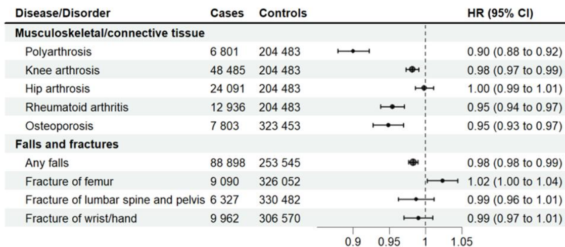
Figure 3. PRS HGS as a predictor of musculoskeletal and connective tissue diseases, falls, and fractures. Multivariable Cox regression analysis. Adjusted for sex, collection year, genotyping batch, and ten principal genetic components of ancestry. HR=hazard ratio, CI=confidence interval.
