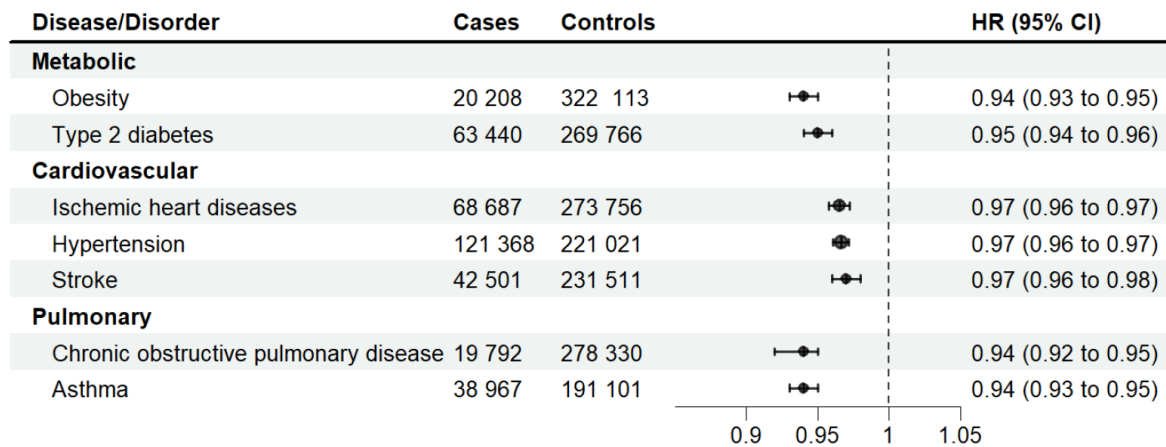
Figure 2. PRS HGS as a predictor of cardiometabolic and pulmonary diseases. Multivariable Cox regression analysis. Adjusted for sex, collection year, genotyping batch, and ten principal genetic components of ancestry. HR=hazard ratio, CI=confidence interval.
