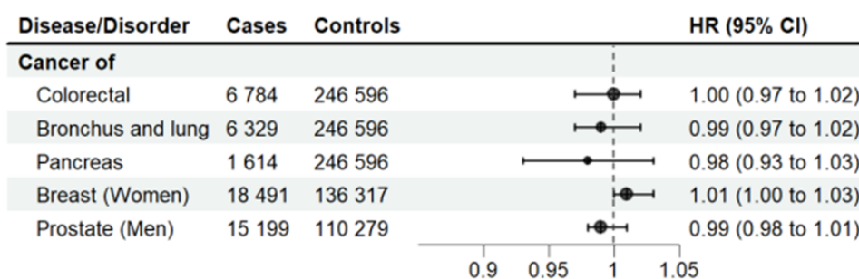
Figure 5. PRS HGS as a predictor of common cancers. Multivariable Cox regression analysis. Adjusted for sex, collection year, genotyping batch, and ten principal genetic components of ancestry. HR=hazard ratio, CI=confidence interval.
