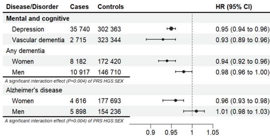
Figure 4. PRS HGS as a predictor of mental and cognitive disorders. Multivariable Cox regression analysis. Adjusted for sex, collection year, genotyping batch, and ten principal genetic components of ancestry. Results with a significant interaction effect ( P < 0.05 ) between PRS HGS and sex are presented stratified by sex. HR=hazard ratio, CI=confidence interval.
