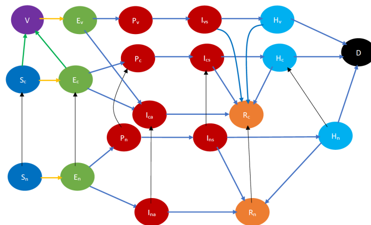
Fig 15. COVID-19 state diagram for two-dose vaccine. The state in purple color is the vaccinated state. The states in blue color are the susceptibles while those in light green color are exposed (still in the incubation period). The states in dark red are infected and therefore infectious while those in gold have recovered, those in light blue are hospitalized, and black denotes dead. In addition, the green arrows denote transition to the vaccinated state after receiving the vaccine, the yellow arrows show susceptibles transitioning to the exposed state after contracting the virus, the black arrows indicate opinion evolution, and the blue arrows indicate the natural progression of the disease. The yellow arrows show susceptibles transitioning to the exposed state after contracting the virus.
