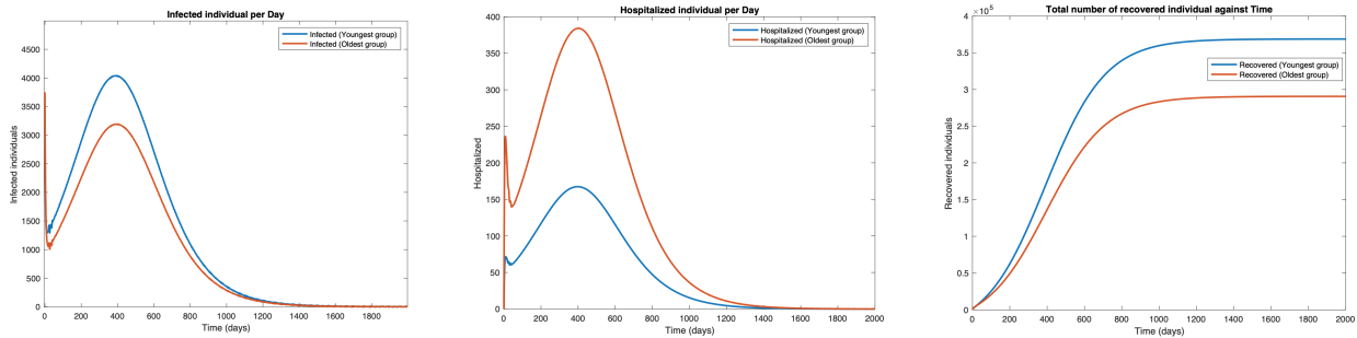
(a) Infection per day (b) Hospitalization per day (c) Number of recovered individuals Fig 5. Scenario 3. Plots in the time domain for sanity check.
