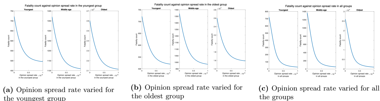
Fig 8. Fatality count when the interaction rates of the oldest group equal that of the youngest group.
