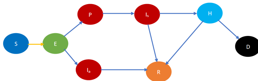
Fig 1. Fundamental COVID-19 state diagram. The states in blue color are the susceptibles (not yet infected but they are prone to infection) while those in light green color are exposed (still in the incubation period, hence they are not infectious). The states in dark red are infected and therefore infectious while those in gold have recovered, those in light blue are hospitalized, and black denotes dead. In addition, the yellow arrows show susceptibles transitioning to the exposed state after contracting the virus. The blue arrows indicate the natural progression of the disease.
