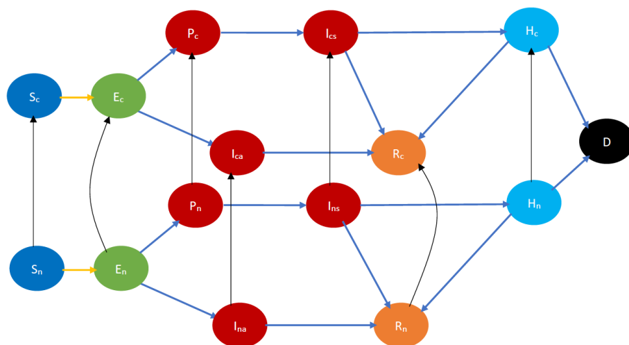
Fig 3. COVID-19 state diagram incorporating cooperativity. The black arrows indicate opinion evolution. The subscript c and n respectively denote cooperative and non-cooperative individuals. Thus, the black arrow from S_n to S_c represents the conversion of a susceptible non-cooperative to a susceptible cooperative, i.e., evolution of opinion of a susceptible. Every state and transition has the same meaning as described in the caption for Fig 1.
