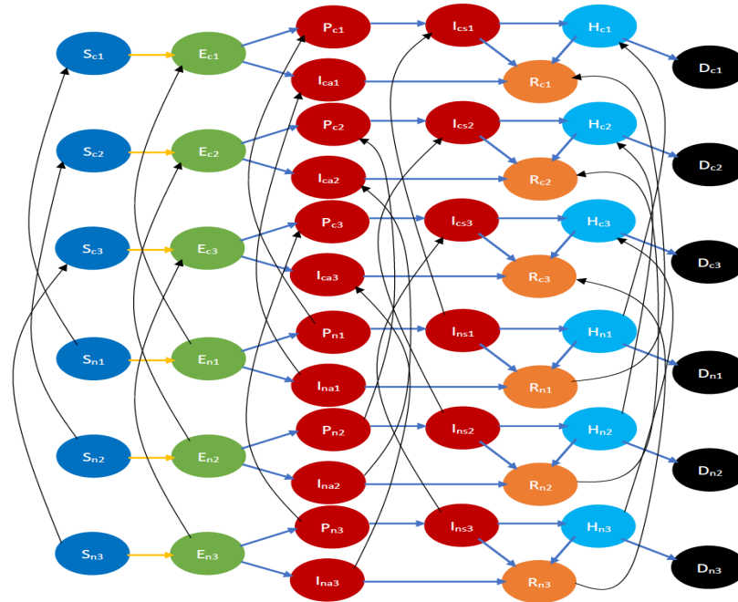
Fig 4. COVID-19 state diagram classified by ages and cooperativities. The subscript c and n respectively denote cooperative and non-cooperative individuals. Similarly, subscripts 1, 2, and 3 represent the youngest group, the middle age group, and the oldest group respectively. Note that there is no transition across age groups, but there is a transition across opinion groups, e.g., there is a transition from S_{n1} to S_{c1} , but no transition between S_{n1}, S_{n2} , or S_{c1}, S_{c2} . Every state and transition has the same meaning as described in the caption for Fig 1.
