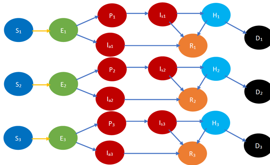
Fig 2. COVID-19 state diagram divided into various age groups. The subscripts 1, 2, and 3 represent the youngest group, middle age group, and oldest group respectively. Every state and transition has the same meaning as described in the caption for Fig 1. Note that there is no transition between states indexed 1, 2, 3, e.g., between S_1, S_2, S_3 as we don't consider transitions between age groups in the time frame under consideration.
