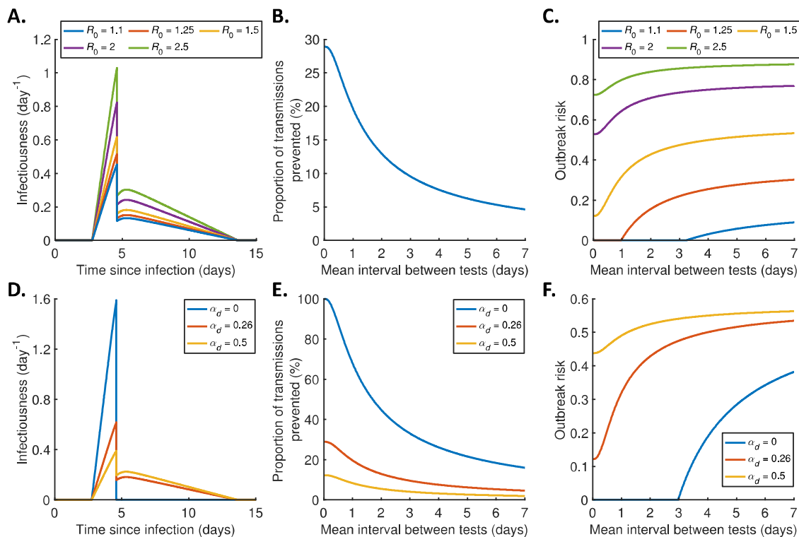
Figure 3. Effect of the local reproduction number and the extent of transmission following detection on the outbreak risk under regular antigen testing. A. Infectiousness profiles without regular antigen testing, assuming a basic reproduction number for local transmissions (in the absence of testing) of R_0 = 1.1 (blue), 1.25 (red), 1.5 (orange), 2 (purple), or 2.5 (green). B. The proportion of transmissions prevented from each infected individual by regular antigen testing (which is independent of R_0 ). C. The outbreak risk for different values of the (mean) interval between antigen tests, plotted for each R_0 value. D. Infectiousness profiles without regular antigen testing, assuming the relative infectiousness of a detected host (compared to an undetected individual with the same viral load) is \alpha_d = 0 (blue), 0.26 (red; the value used elsewhere in our analyses (44)), or 0.5 (yellow), with R_0 = 1.5 in all cases. Under these \alpha_d values, the proportions of presymptomatic transmissions (without regular antigen testing) are 100%, 39% and 25%, respectively. E. The proportion of transmissions prevented from each infected individual by regular antigen testing, for different values of the (mean) interval between tests, plotted for each \alpha_d value. F. The outbreak risk for different values of the (mean) interval between tests, plotted for each \alpha_d value.
