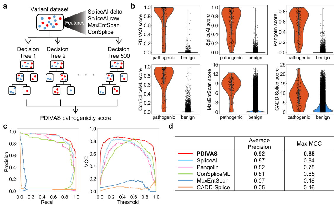
Fig. 2 PDIIVAS outperforms the existing predictors in classifying pathogenic and benign variants.
