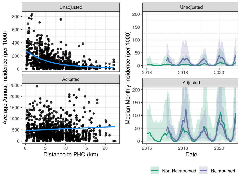
487 488 Figure 3. The ZERO-G adjustment method greatly reduces geographical and financial 489 bias in malaria incidence rates. Left: Each point represents the average annual malaria 490 incidence rates for a fokontany over the period of 2016-2020, with the x-axis showing the 491 distance to the nearest PHC. The smoothed line is the exponential (unadjusted) or linear 492 (adjusted) fit between average annual incidence and distance to PHC. One outlier point is 493 removed to aid with visualization. Right: The median monthly malaria incidence rates across 494 fokontany whose closest PHC does or does not offer fee reimbursement. Fee reimbursement 495 began in January 2017. The error ribbon represents a 90% CI. The y-axis is limited between 496 values of 0-200 to aid with visualization. 497
