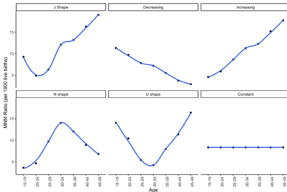
Figure 1 Simulated MNM age distributions
