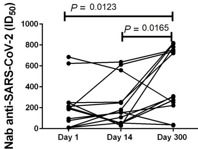
681 Figure 3: Longitudinal humoral immune response of inpatients with COVID-19. A, 682 Nabs (ID 50 ) of COVID-19 patients at admission D1 compared to the Nab (ID 50 ) 683 assessment 14 days after hospital discharge. B, Nabs (ID 50 ) of COVID-19 684 patients at admission D1 compared to Nab (ID 50 ) assessment 300 days after 685 hospital discharge. C, Changes in Nab titers (ID 50 ) for each patient are shown 686 over time. Data from patients for the first sample D1, after 14 days and the last 687 collected sample D300 are shown.
