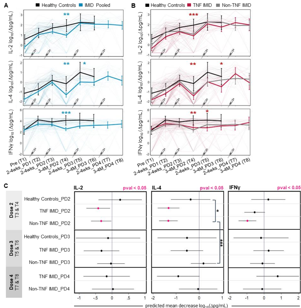
Figure 6. Longitudinal analyses of T cell cytokine responses pre and post one to four doses of SARS-CoV-2 mRNA vaccine. Timepoints are defined in Table 1. (A, B) Predicted mean T cell cytokines IL-2, IL-4, IFN \gamma ( \log_{10}(\Delta pg/mL) ) from pre-vaccination to after one to four doses of vaccine. Mixed-effects linear regression models controlled for age, BMI, and sex, with an interaction term between timepoint and group (thick lines). Individual patients are plotted in thin lines. Groupings: healthy controls (black), IMID patients pooled (blue), TNF IMID (anti-TNF or anti-TNF+MTX/AZA treated) patients (red), and IMID patients not treated with anti-TNF (grey). An additional control for vaccine type was incorporated into mixed-effects regression models to compare groups: a) IMID pooled vs healthy controls (blue asterisks) or b) TNF IMID vs healthy controls (red asterisks). (C) Predicted mean decrease of T cell cytokines IL-2, IL-4, IFN \gamma ( \log_{10}(\Delta pg/mL) ) in healthy controls, TNF IMID, and IMID patients not treated with anti-TNF between 2-4 weeks and 3-4 months after dose 2 (decrease between T3 and T4), after dose 3 (decrease between T5 and T6), and after dose 4 (decrease between T7 and T8). Mixed-effects linear regression models controlled for age, BMI, sex, vaccine type, with an interaction between timepoint and group. Mean decrease values that are significant ( p_{val} < 0.05 ) are colored in pink. Significant pairwise comparisons are indicated by asterisks and brackets. (A-C) Sample sizes are listed in Supplemental Table 1. * p < 0.05 ; ** p < 0.01 ; *** p < 0.001 ; \Delta : background subtracted; pg/mL: picogram per milliliter; PD: post dose
