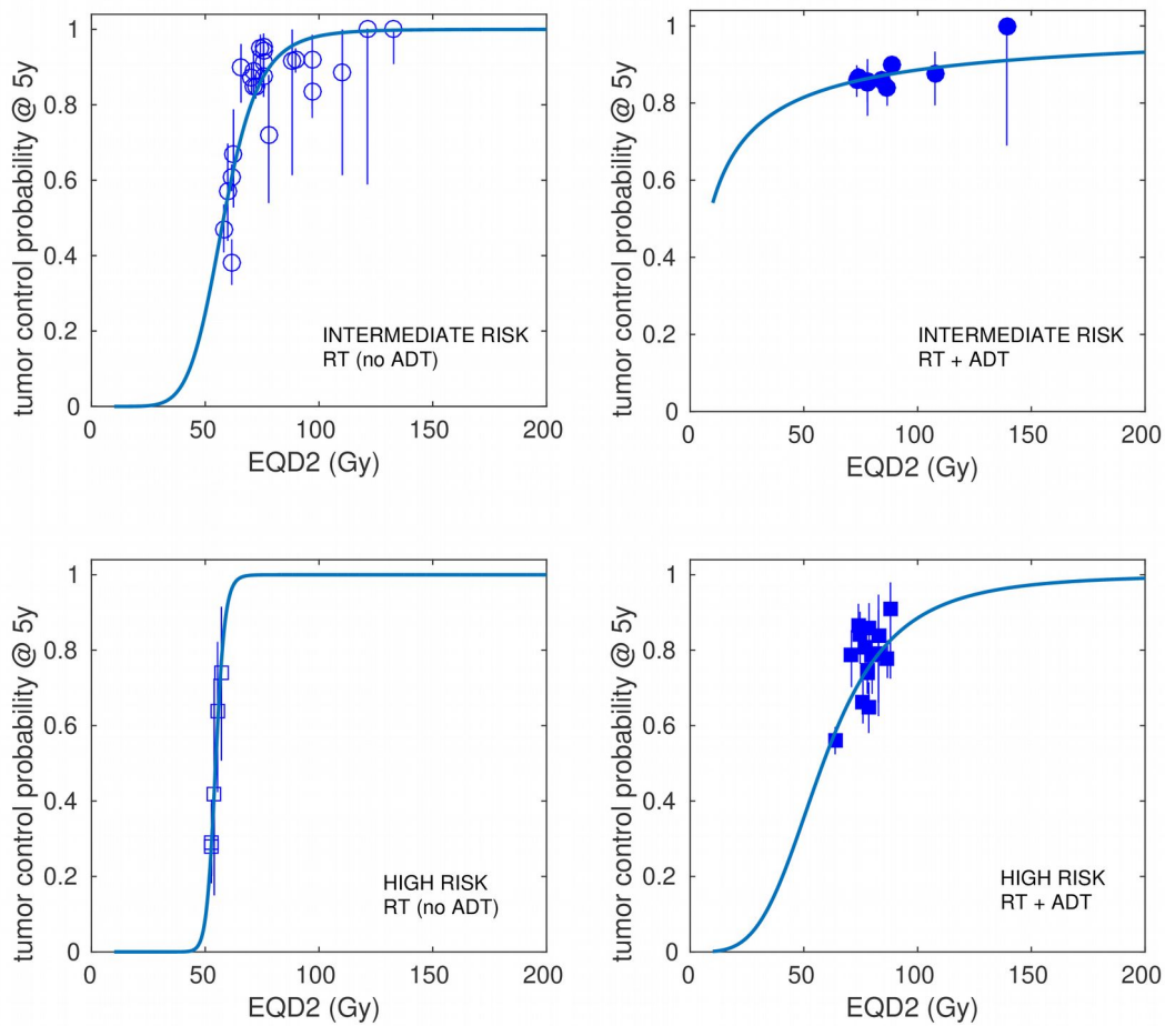
Figure 2: Best fits to intermediate- and high-risk prostate carcinoma dose-response data obtained with the linear quadratic model. Results are presented separately for cohorts that use androgen deprivation therapy (ADT) and cohorts not using ADT in addition to radiotherapy.
