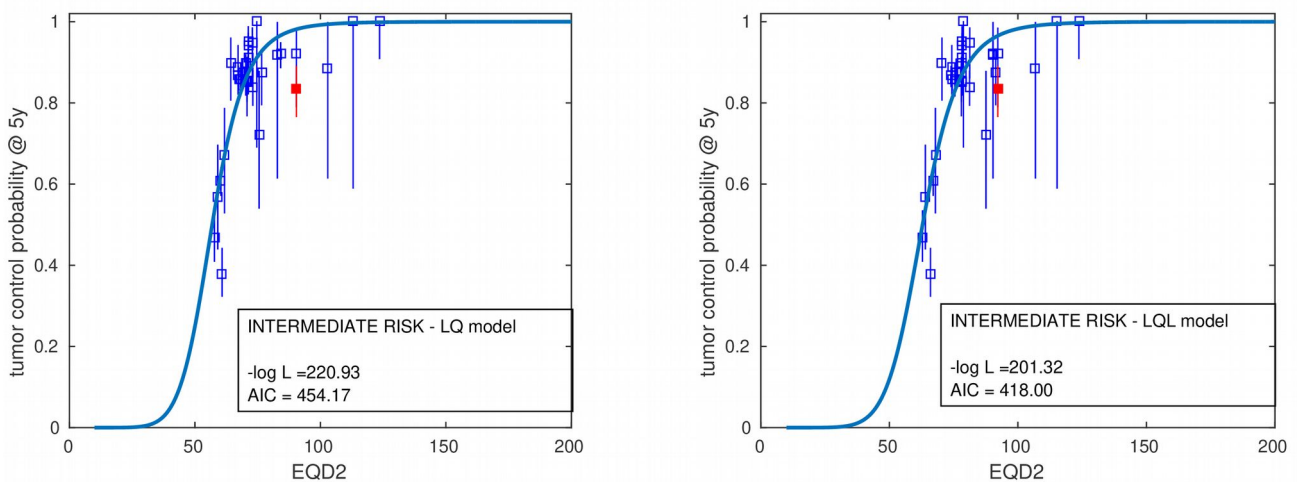
Supplementary Figure 2: Best fits to intermediate risk dose-response data for prostate cancer obtained with the linear quadratic (LQ) and linear-quadratic-linear (LQL) models: left panel and right panel, respectively. In red we highlight the schedule that conditions the superiority of the LQL model: reported by Levin-Epstein et al. , it includes 157 intermediate risk patients treated with 38 Gy in 4 fractions (9.5 Gy per fraction), and control at 5 years was 83.6%
