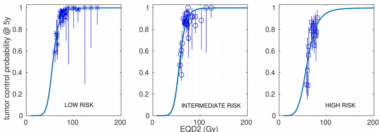
Figure 1: Best fits to prostate carcinoma dose-response data obtained with the linear quadratic model. Results are presented separately for low risk (left panel), intermediate risk (central panel) and high risk (right panel).
