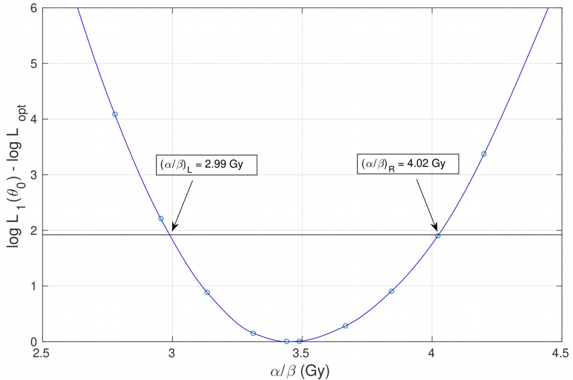
Supplementary Figure 1: Illustration of the calculation of 95% confidence intervals for the parameter (\alpha/\beta) in IR patients.
