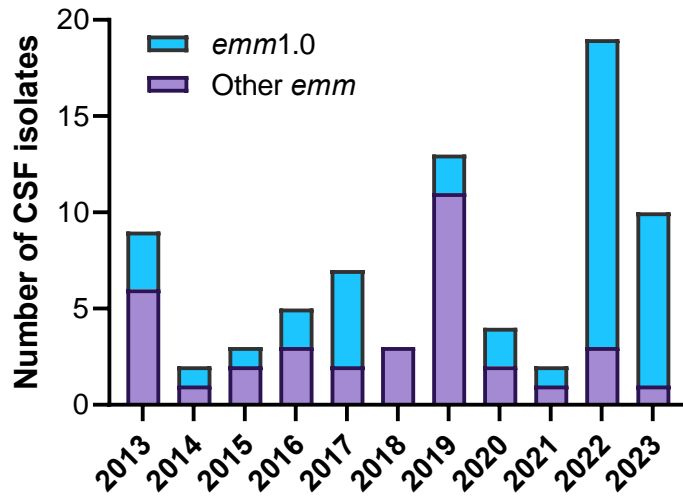
Figure 1. Number of received S. pyogenes CSF isolates with proportion of emm1.0 , 2013-2023 (until March 13 th ).
