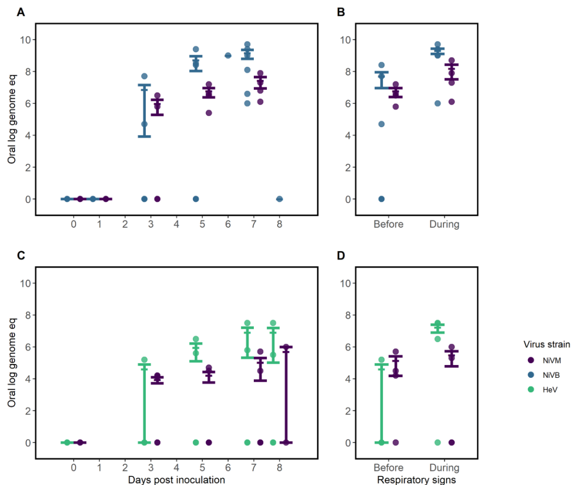
Figure 5. Comparing virus quantity in oral samples of African green monkeys infected with Hendra virus (HeV) or Nipah virus Bangladesh (NiV B ) compared with Nipah virus Malaysia (NiV M ) in studies with similar study protocols, by route of inoculation. (a) Virus quantity by days post inoculation and (b) peak quantity before and during respiratory signs in animals inoculated intratracheally with NiV M and NiV B 26,27 (N=9). (c) Virus quantity by days post inoculation and (d) peak quantity before and during respiratory signs in animals inoculated intranasally/intratracheally 28,29 with NiV M and HeV (N=11). Quantities are shown as log genome equivalents. Error bars represent mean and standard error. Four African green monkeys were excluded from b and d as no samples were positive by PCR and/or the animals did not develop respiratory signs.
