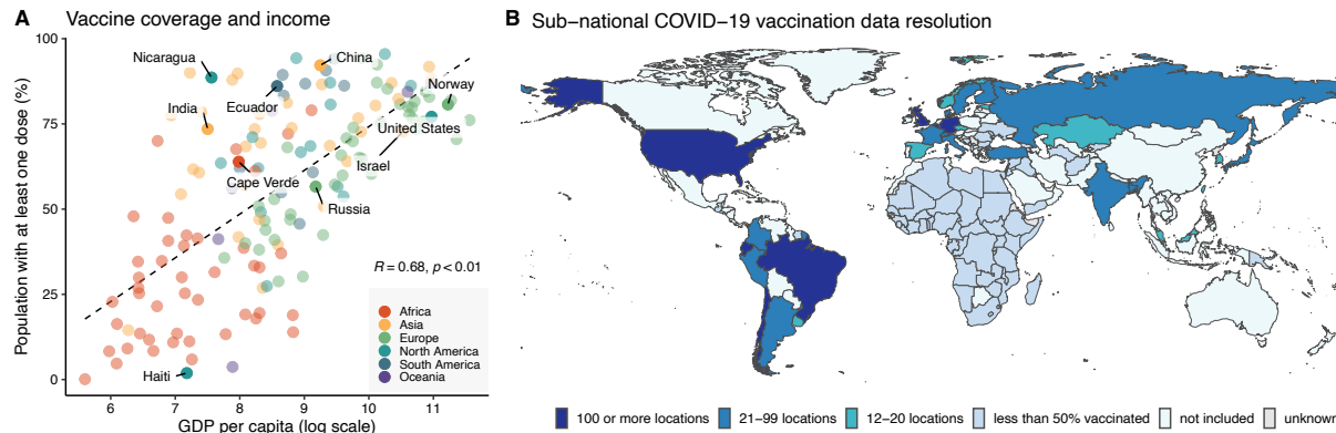
Figure 1: SARS-CoV-2 vaccine coverage. (A) Association between population vaccinated with at least one dose and gross domestic product (GDP) per capita for 160 countries and territories. Vaccine and population data come from [23–55] and were compiled by the Financial Times as of June 22, 2022. GDP data are sourced from World Bank [56] and PCBS [57]. (B) Sub-national vaccination data resolution. Based on publicly available data for places with 50% or more of their population vaccinated with at least one dose, we identified 7 countries/territories with vaccination rates for 100 or more locations, 17 for 21-99, and 10 for 12-20 locations. In this study, we excluded 78 countries that have greater than 50% vaccination coverage due to a lack of high-resolution sub-national data, which are referenced as ‘not included’ in the legend. Details of the data sources and dates of data collection are reported in tables S1 and S2, respectively.
