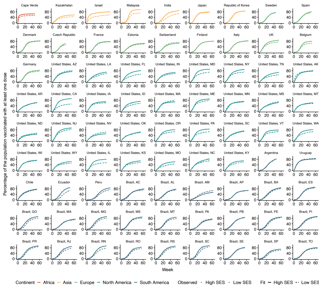
Figure 2: Observed (points) and predicted (lines) temporal trends of first-dose COVID-19 vaccine coverage at the sub-national level for high (solid) and low (dashed) SES groups, spanning 26 countries. A remaining 9 places are analyzed in figure S1, and full list of excluding factors are described in the supplementary text. Week 0 is the first week available in the data.
