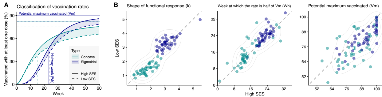
Figure 3: Parameters from the functional response fitting and the two temporal trends identified using the Gaussian mixture model [61]. (A) Vaccination trends over time for concave (teal) and sigmoidal (purple) types. The percentage of the cumulative population vaccinated over time for each type and SES (low in dashed line and high in solid line) were calculated using the average parameters for each type based on the classification of the 81 locations shown in figure 2. Parameters for each place can be found in table S4. (B) Values for low and high SES of the shape parameter k , the week at which half of the vaccination potential is reached W_h , and of the potential maximum percentage of the population vaccinated V_m , colored by the two temporal trends. Clustering is still apparent when displaying the United States and Brazil as countries rather than states (fig. S11).
