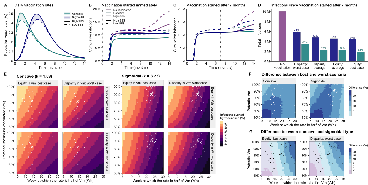
Figure 4: (A) Average daily vaccination rates for each type and SES group (per-country rates shown in fig. S13). In the sigmoidal type, the parameters for high SES are V_m = 89\% and W_h = 23 weeks, while for low SES are V_m = 82.5\% and W_h = 24 weeks. For both SES groups, k = 3.23 , the average across SES. In the concave type, the parameters for high SES are V_m = 82.2\% and W_h = 14 weeks while for low SES they are V_m = 75.5\% and W_h = 15 weeks. For both SES groups, k = 1.58 . (B) Cumulative cases per 10,000 with vaccination starting immediately. (C) Cumulative cases per 10,000 with vaccination starting at t = 7 months. (D) Cumulative cases per 10,000 after 14 months under 4 scenarios of socioeconomic disparity: disparity: average, disparity: worst case (95th percentile), equity: average (averaging high SES and low SES parameters), and equity: best case (assuming vaccination of the low SES group follow the same parameters as the high SES group). (E) Cases averted by vaccination. Keeping k = 1.58 for concave and k = 3.23 for sigmoidal, we fixed the low SES parameters at a constant disparity from high SES based on the 95th percentiles of the observed data ( \Delta V_m = 21\% , \Delta W_h = 6 weeks), or considered low SES parameters equal to high SES (equity) (fig. S16). The effect of varying parameter k can be found in figure S17. (F) The difference in cases averted under the best-case equity scenario and worst-case disparity, for both concave and sigmoidal types. (G) The difference in cases averted under concave versus sigmoidal types, for both best-case equity and worst-case disparity. Average high SES parameters are illustrated with a cross, while country-specific parameters for high SES are shown with dots. Model parameters are listed in table S5.
