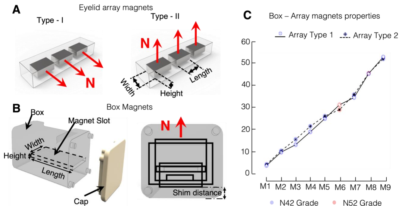
Figure 1 | Experimental setup to study the effect of increasing magnetic force on blink dynamics (Box Experiment). A , Eyelid array magnets are small (L x W x H: 3 x 2 x 1mm) rectangular magnets embedded in PDMS that is bonded on IV 3000 skin adhesive film. As shown by the red arrows, Type-I arrays have the manufacturer-defined magnetization orientation along the height of the magnets while Type-II have magnetization orientation through the width (SM magnetics, Pelham AL, USA), dot marker on denoted pole. B , Boxes had a slot where rectangular static Neodymium grade 42 or 52 magnets (M1 to 9) were inserted to produce magnetic surface force ranging from 5 to 55gF in 5-10gF increments, verified with strain gauge. Shims were used to make minor adjustments in surface force as needed. All boxes (M1-9) looked identical and were arbitrarily labeled to mask the operator and participant to size and force. The north pole of the box magnet was oriented upwards such that the north pole of the array was attracted to the bottom of the box. Black outlined rectangles represent the cross-sectional geometries of the various boxes. C , Surface pull force for each box. The y-axis represents empirical measurements of surface pull force in grams (gF) exerted on the type I and II arrays, measured with a strain gauge.
