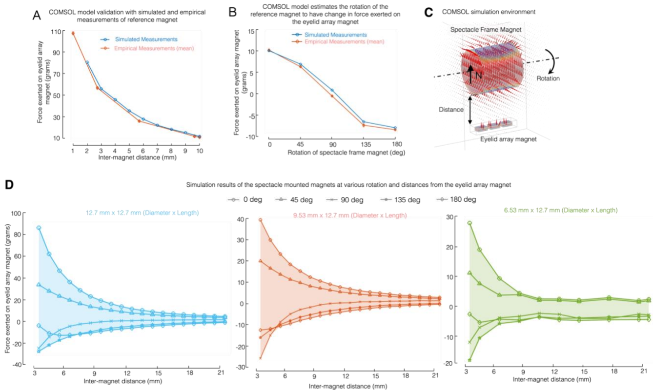
Figure 4: COMSOL model validation and simulated results for force modulation using angular translation, inter-magnet linear distance translation, and spectacle magnet diameter variation. A , Line plot showing minimal difference between empirical and COMSOL simulated force measurements. Measurements represent forces of a diametrically magnetized N52 reference magnet (12.7mm x 12.7mm cylindrical magnet) on a type II eyelid array. The eyelid array reference magnet were placed at various predefined distances [1mm – 10mm] (x-axis) and force acting on the top surface of the eyelid array magnets was measured 3 times each with a strain gauge (y-axis). B , Line plot showing minimal difference between COMSOL simulated and empirical force measurements of force variation (y-axis) with spectacle magnet angular translation (x-axis), validating the COMSOL model. Measurements represent the forces of a diametrically magnetized reference magnet with the type-II eyelid array magnet separated at a distance of 10mm. At 0° both magnets poles are aligned in the same direction (reference magnet south pole is aligned with eyelid array magnets north pole). The reference magnet was rotated by 45° steps from 0 to 180 degrees and force was measured 3 times each with a strain gauge. C , COMSOL model used for simulation of the environment of the spectacle frame magnet or reference magnet and the eyelid magnet array. The eyelid array was simulated as encapsulated in the PDMS substrate. The space between the eyelid array magnet and the spectacle frame magnet is simulated as air. D , Line plots reporting the results of simulations. Three magnet sizes were simulated while varying the angle of the spectacle magnet (y-axis) and inter-magnet distance(x-axis). Rotation angles were simulated at 45° steps. The shaded region represents the range of forces that can be exerted by the spectacle magnet on the type II eyelid array magnet due to a change in inter-magnet distance and angular rotation. Negative force values represent repulsion and positive force values represent attraction.
