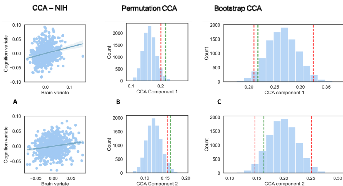
Figure 2. Results of the CCA analyses. A.1-2. Canonical correlation plots between the cerebellar and clinical variates. B.1 - B.2 Significance testing of the CCA. Distribution of CCA coefficients for component 1 (B.1) and component 2 (B.2) obtained by performing 10'000 permutations. Red line represents a significance threshold set for an alpha level of 0.05. C.1-C.2. Stability testing of the CCA. Distribution of canonical correlation coefficients between cerebellar and clinical variates by bootstrapping procedure with 10 '000 tests at an alpha level of 0.05 for component 1 (C.1) and component 2 (C.2). Lower and upper bound corresponding to \pm 1.96 SD in red dotted line
