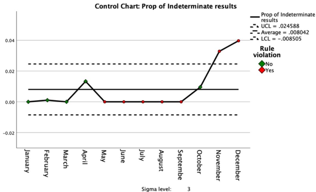
Figure 1. Control chart with five successive points on the same side of the centerline
