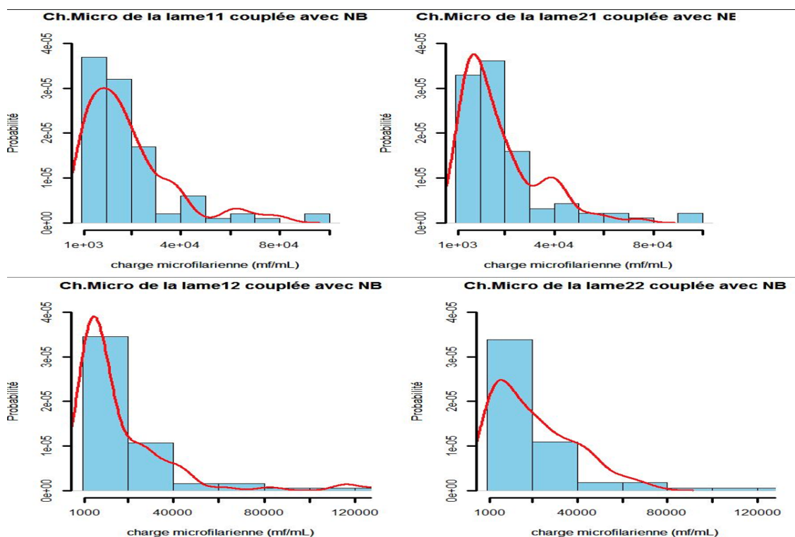
Figure 2: Adaptation of the negative binomial law of parameters (a, \lambda) to the microfilar charge of Loa loa whose parameters are on the table 1 as a function of the blade
