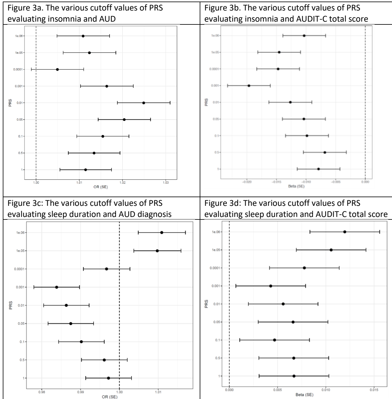
Figure 3: Polygenic Risk Score Analysis of sleep- and alcohol-related variables
