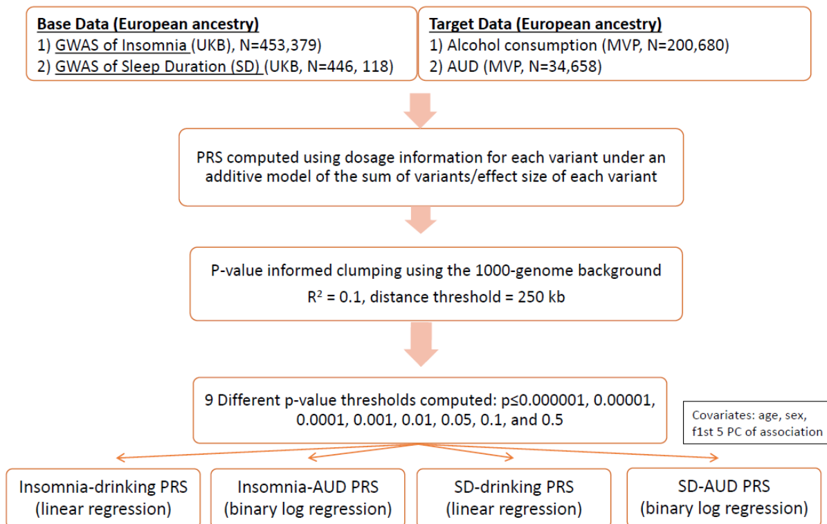
Figure 1. PRS methodology in the current study
