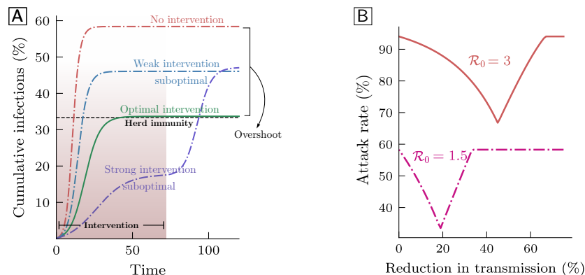
FIG. 1. (A) Simulation of four types of intervention for an epidemic with \mathcal{R}_0 = 1.5 in a homogeneous population: (i) No intervention – leads to largest attack rate, (ii) Weak intervention – reduces the attack rate, (iii) Strong intervention – reduces attack rate during the intervention, but leads to a resurgence in infections once the intervention is removed, (iv) A moderate intervention but optimal – attack rate is same as the herd immunity threshold. (B) The existence of a global minima for the attack rate shows that an optimal intervention strength exists. The resurgence of infections under a strong sub-optimal intervention is subject to certain assumptions which are discussed in section IV.
