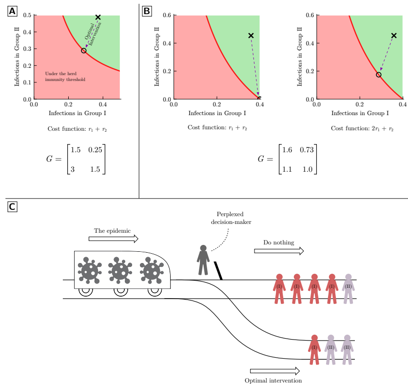
FIG. 2. Population structure and non linearity of infectious disease dynamics lead to an ethical dilemma. (A) A plot of the infections in the two groups that constitute the population. The corresponding cost function and next generation matrix are shown. The red curve shows the herd immunity threshold, the point marked with a cross shows the attack rate without an intervention, the point marked with a circle shows the attack rate if the optimal intervention is used. (B) A comparison of the interventions when the cost functions are different. The first plot shows that the optimal intervention leads to an increase in the number of infections in the first group. It is an example of the ethical dilemma of implementing the optimal intervention, which is explained further in (C) . The second figure shows the plot for the cost function when the first group is given twice the weight as the second group, which means prevention of infections in the first group takes precedence over the second group. In this case, the intervention reduces the infections in both the groups. Thus, a biased cost-function may allow us to avoid the ethical dilemma. (C) This figure shows that the ethical dilemma involved in implementing optimal interventions is analogous to the well-known ‘trolley problem’. If the decision-maker does not act, the incoming epidemic (represented as a trolley) is going to cause many infections. If the decision-maker implements an optimal intervention (switches the tracks), the number of infections in the total population is minimised, but someone who otherwise would have been safe from infection, becomes infected (shown by the increased number of infections of group (II)).
