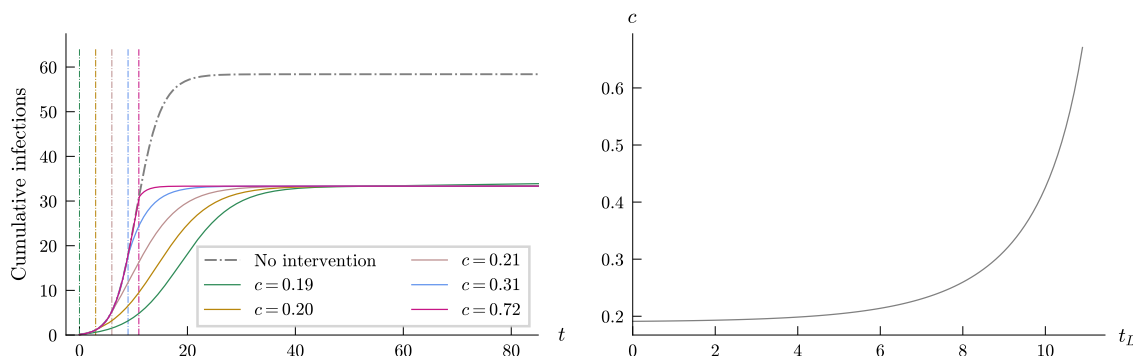
FIG. 3. Left: The time series of cumulative infections ( i + r ) for optimally controlled epidemics for a range of delays in the intervention. The vertical dash-dot lines show the time at which the intervention starts, and its corresponding time series is represented by the same color. Right: The strength of optimal intervention c plotted against the delay in intervention t_L using equation (9). The super-linear increase in c shows the need for an early implementation. Parameters: Homogeneous SIR model with basic reproduction number \mathcal{R}_0 = 1.5 and \gamma = 1 . Intervention is implemented for a duration of 50 time units.
