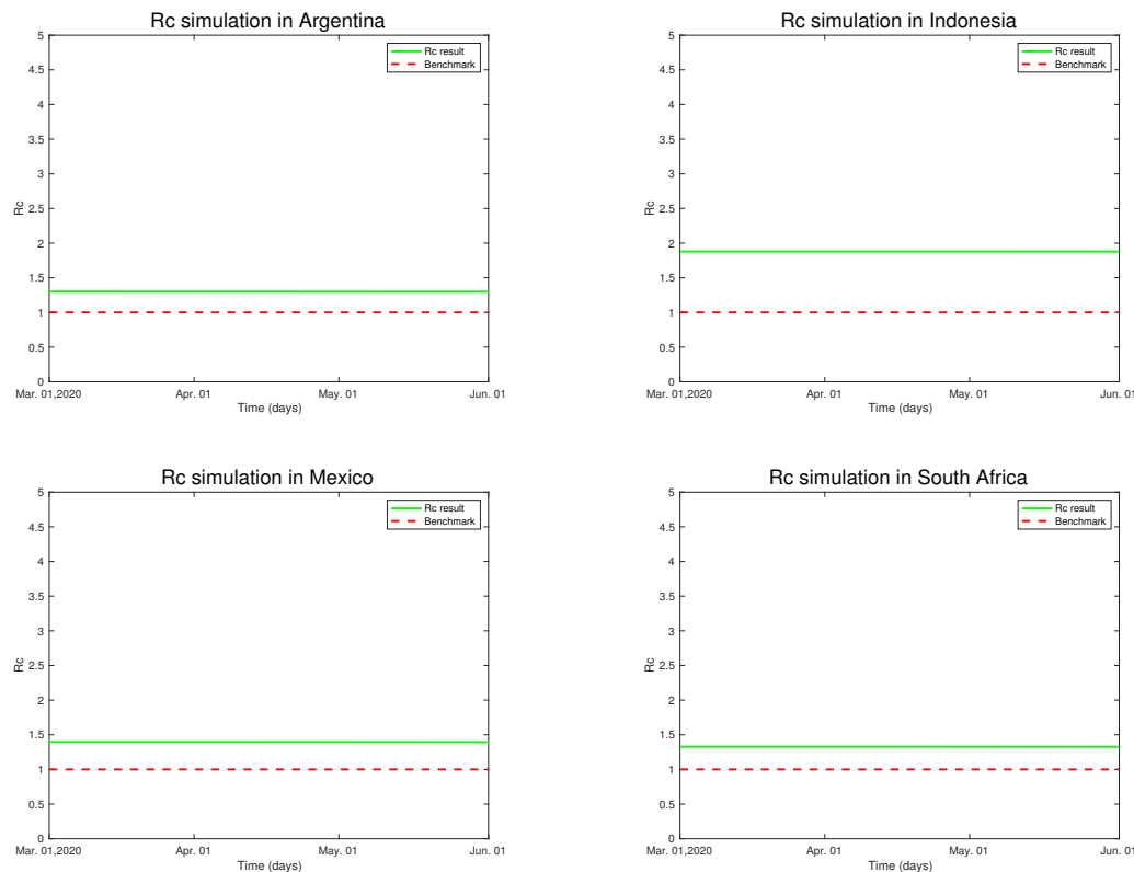
Figure 7: Results of the basic reproduction numbers
