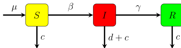
Figure 2: Flowchart of SIR model with birth and death
