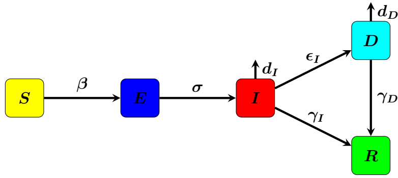
Figure 5: Flowchart of the SEIDR model
