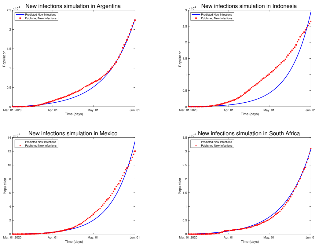
Figure 6: Simulations and real values on new infections
