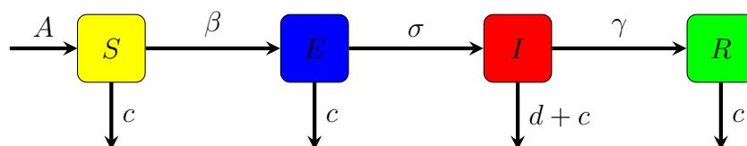
Figure 4: Flowchart of SEIR model with death and migration
