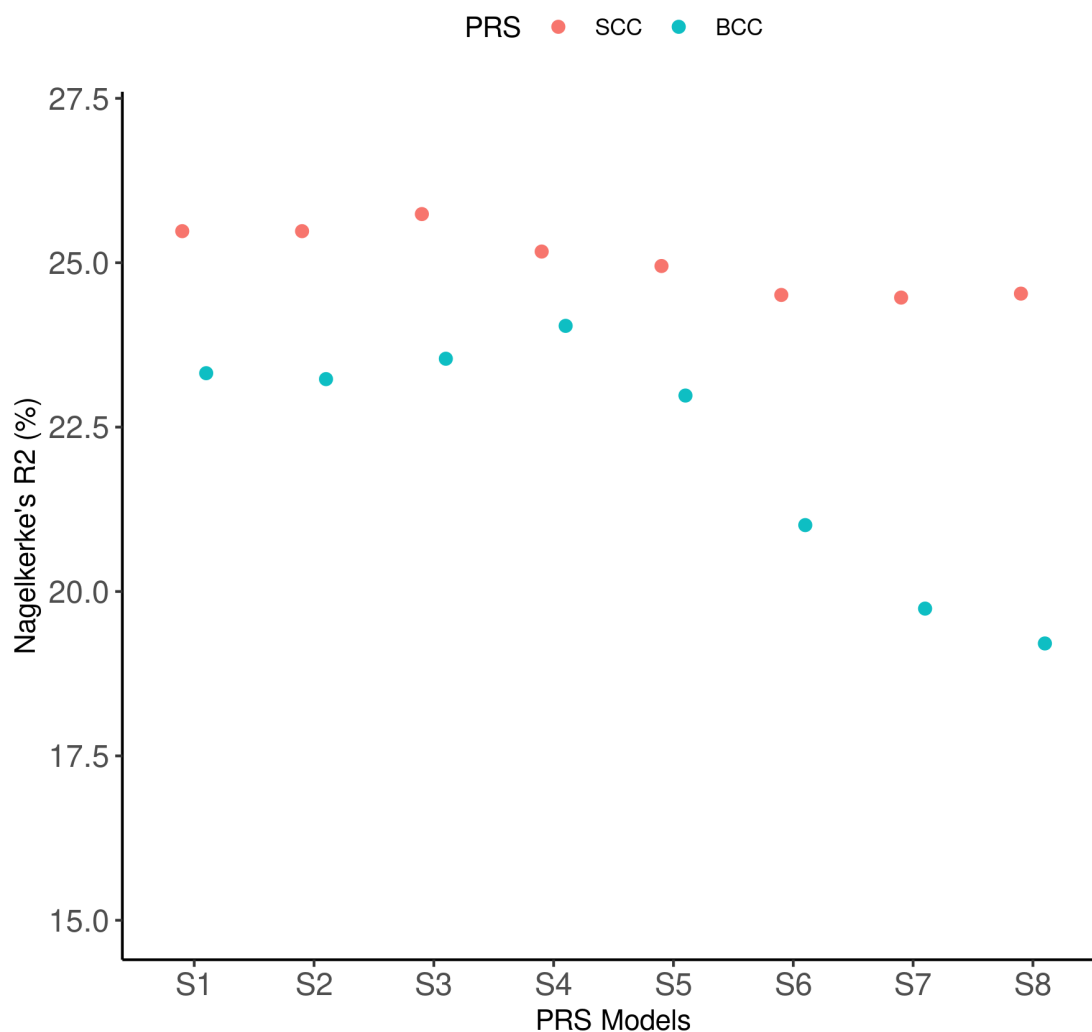
Figure 3 The performance of SCC and BCC PRS prediction models in the validation cohort.
