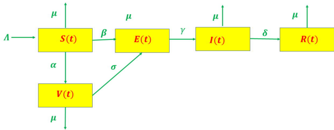
Figure 1. Dynamic transmission model of COVID-19
