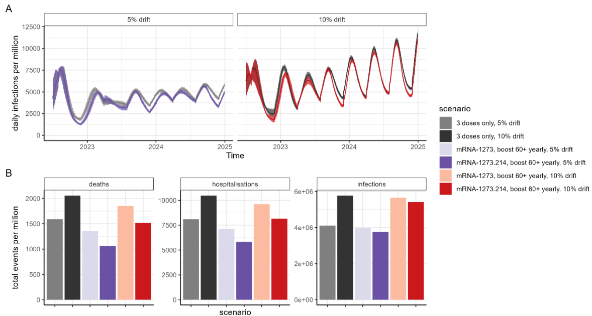
Figure 3: Impact of vaccination in future scenarios where the virus continues to gradually evolve (or "drift"), in a high-income setting with substantial prior transmission (Category 1). This is implemented in the model by increasing both the level of transmission and the VFR relative to Delta every 4 months, to represent both an increase in transmissibility and gradual immune escape. Here we show two levels of transmission and immune escape: 5% (purple/lilac) and 10% (red/orange). (A) Daily infections per million population assuming either 5% or 10% drift, either with the first three doses given only (light and dark grey), or with annual boosting to the 60+ population (purple and red). (B) Total events per million population between 1 July 2022 and end-2024, for the two "drift" scenarios, and for no boosting (light and dark grey) and boosting with either the original mRNA-1273 vaccine (lilac and orange), or with the bivalent mRNA-1273.214 vaccine from dose 4 onwards (purple and red). Results for the Category 2 and 3 settings are in Figures S11–12 .
